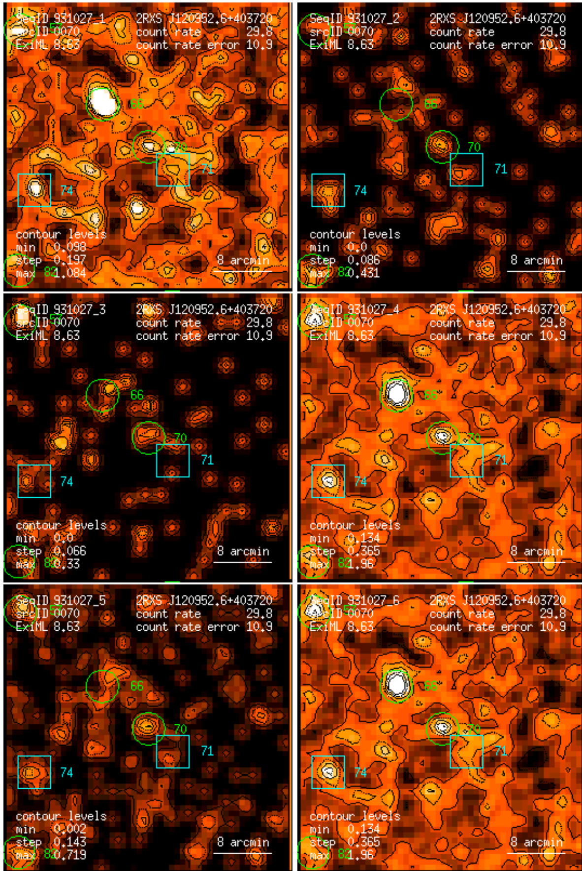
Figure 70: RASS 931027: detection 0070: band rate images, Gaussian filter: (1) PSPC channels 11 – 41, (2) 52 – 90, (3) 91 – 201, (4) 11 – 235, (5) 52 – 201, (6) 11 – 201. Broad band rates in counts/ks. Band rate contour levels in counts/ks/arcmin 2 .
