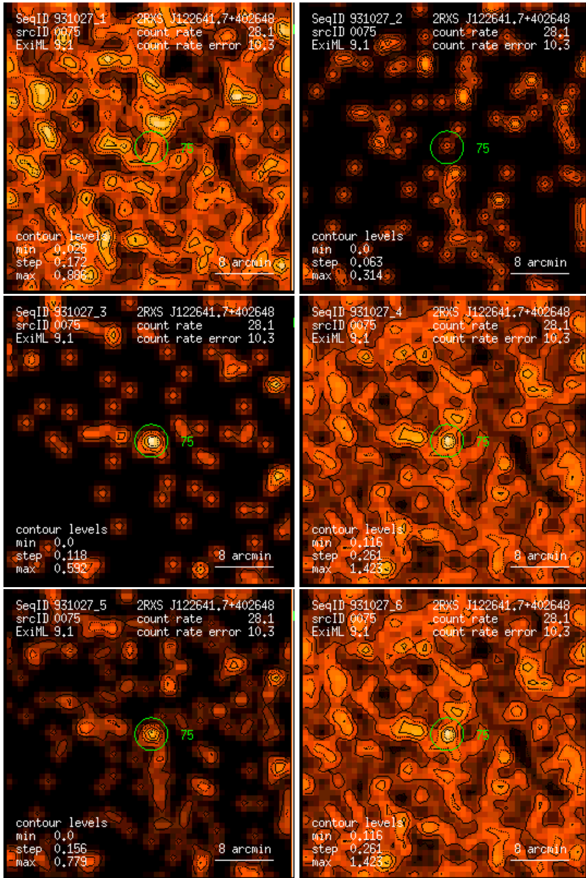
Figure 75: RASS 931027: detection 0075: band rate images, Gaussian filter: (1) PSPC channels 11 – 41, (2) 52 – 90, (3) 91 – 201, (4) 11 – 235, (5) 52 – 201, (6) 11 – 201. Broad band rates in counts/ks. Band rate contour levels in counts/ks/arcmin 2 .
