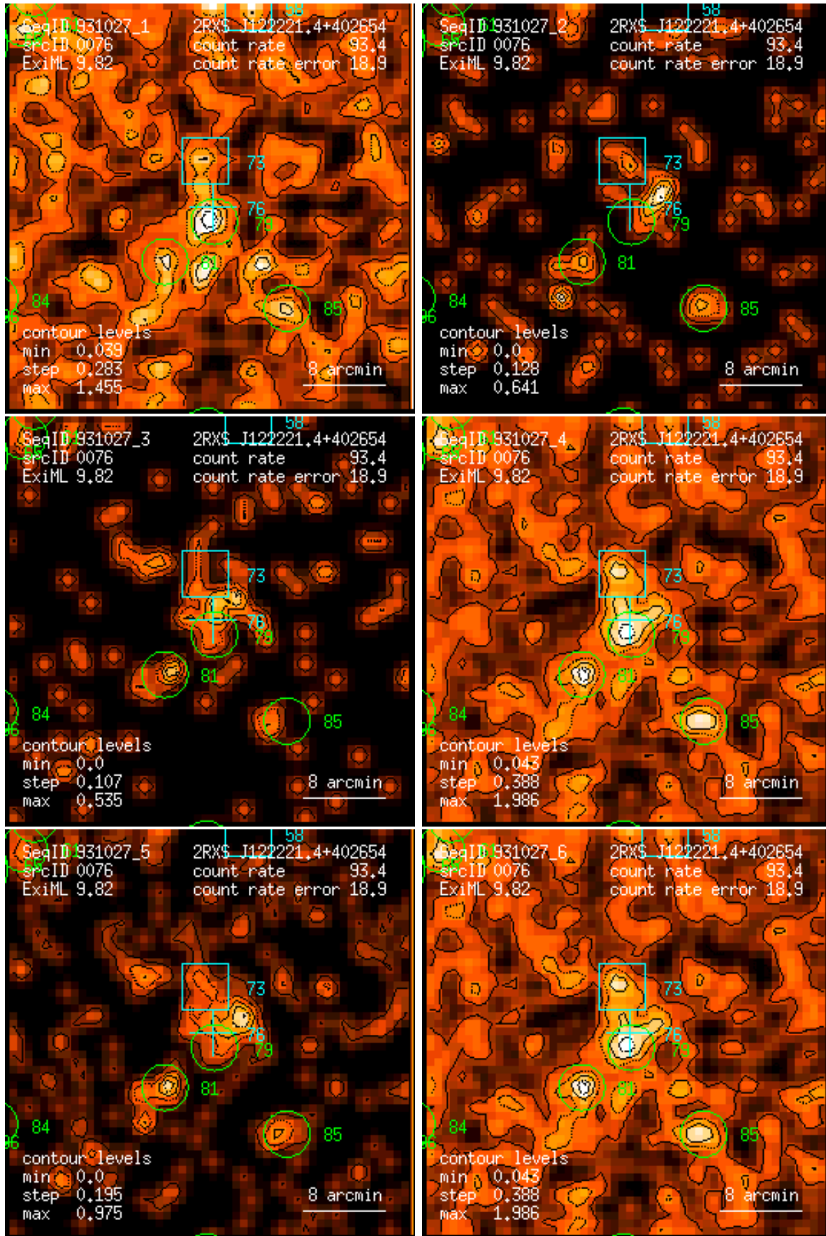
Figure 76: RASS 931027: detection 0076: band rate images, Gaussian filter: (1) PSPC channels 11 – 41, (2) 52 – 90, (3) 91 – 201, (4) 11 – 235, (5) 52 – 201, (6) 11 – 201. Broad band rates in counts/ks. Band rate contour levels in counts/ks/arcmin 2 .
