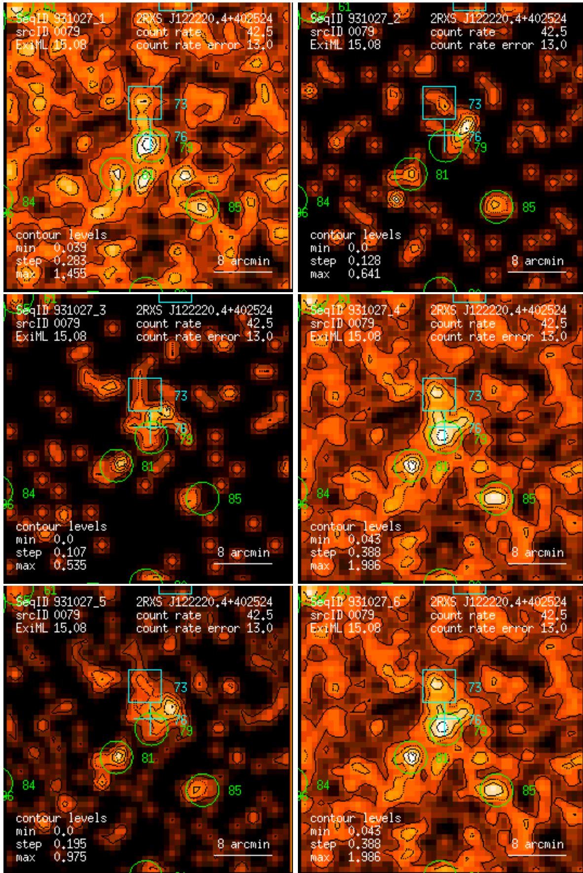
Figure 79: RASS 931027: detection 0079: band rate images, Gaussian filter: (1) PSPC channels 11 – 41, (2) 52 – 90, (3) 91 – 201, (4) 11 – 235, (5) 52 – 201, (6) 11 – 201. Broad band rates in counts/ks. Band rate contour levels in counts/ks/arcmin 2 .
