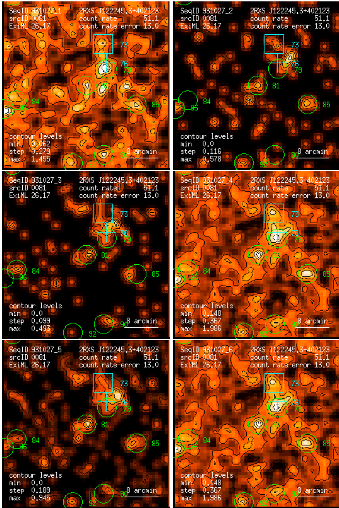
Figure 81: RASS 931027: detection 0081: band rate images, Gaussian filter: (1) PSPC channels 11 – 41, (2) 52 – 90, (3) 91 – 201, (4) 11 – 235, (5) 52 – 201, (6) 11 – 201. Broad band rates in counts/ks. Band rate contour levels in counts/ks/arcmin 2 .
