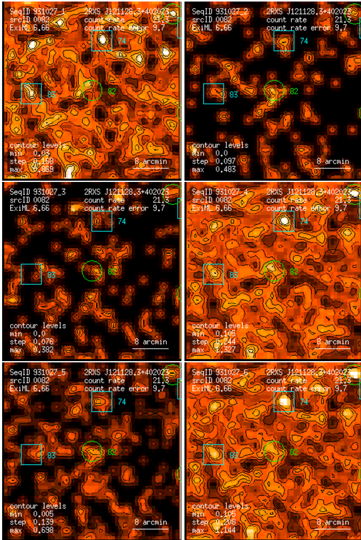
Figure 82: RASS 931027: detection 0082: band rate images, Gaussian filter: (1) PSPC channels 11 – 41, (2) 52 – 90, (3) 91 – 201, (4) 11 – 235, (5) 52 – 201, (6) 11 – 201. Broad band rates in counts/ks. Band rate contour levels in counts/ks/arcmin 2 .
