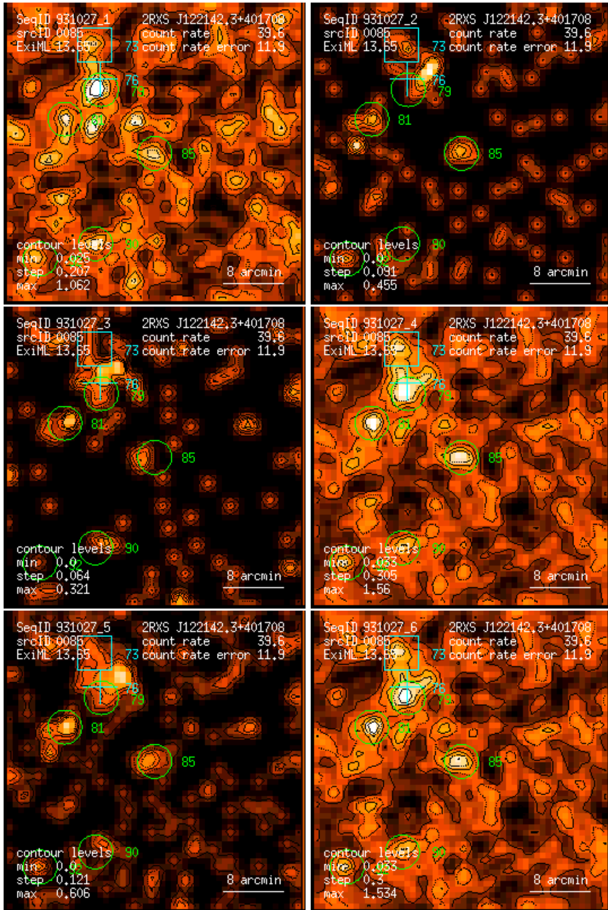
Figure 85: RASS 931027: detection 0085: band rate images, Gaussian filter: (1) PSPC channels 11 – 41, (2) 52 – 90, (3) 91 – 201, (4) 11 – 235, (5) 52 – 201, (6) 11 – 201. Broad band rates in counts/ks. Band rate contour levels in counts/ks/arcmin 2 .
