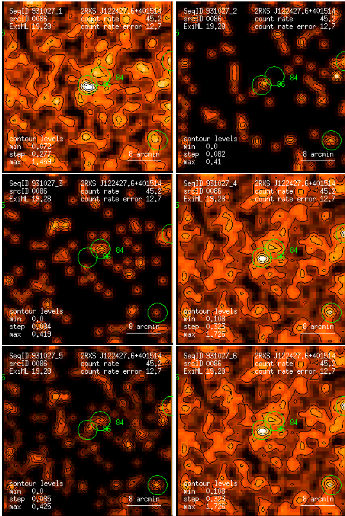
Figure 86: RASS 931027: detection 0086: band rate images, Gaussian filter: (1) PSPC channels 11 – 41, (2) 52 – 90, (3) 91 – 201, (4) 11 – 235, (5) 52 – 201, (6) 11 – 201. Broad band rates in counts/ks. Band rate contour levels in counts/ks/arcmin 2 .
