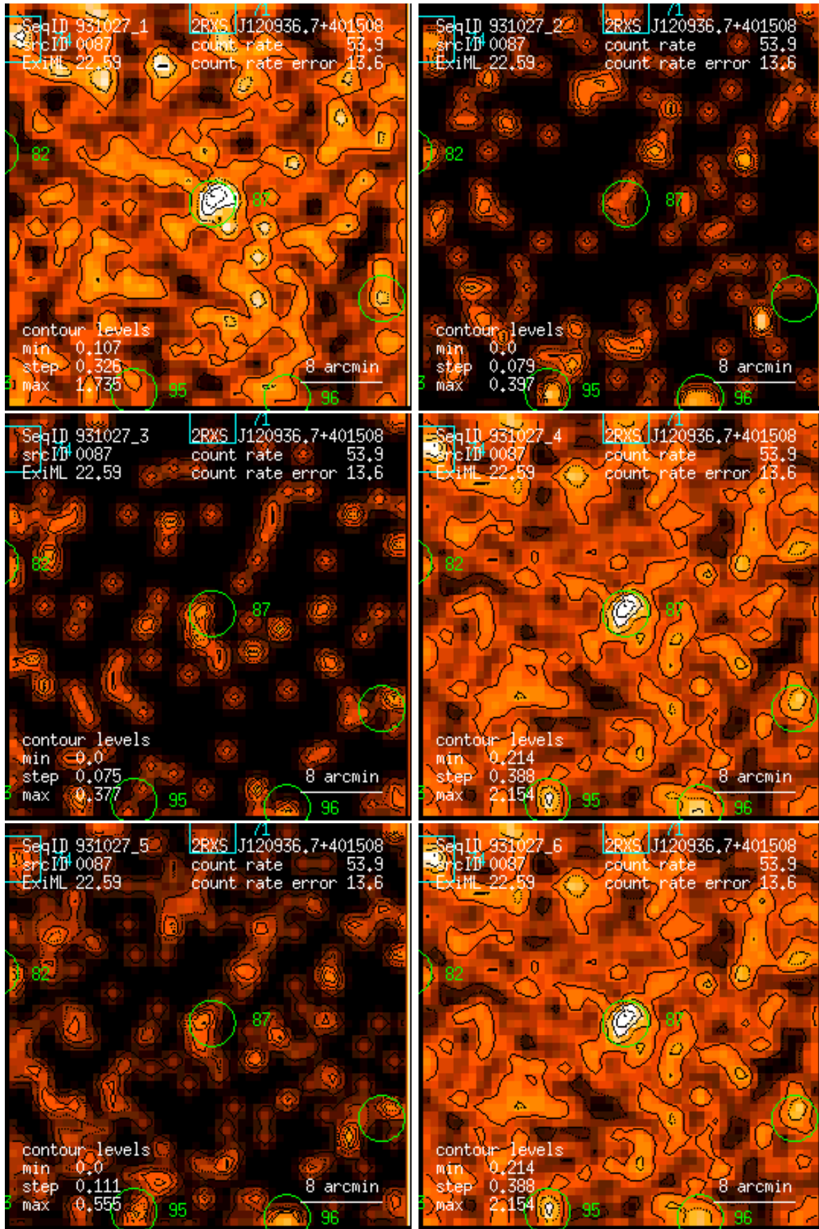
Figure 87: RASS 931027: detection 0087: band rate images, Gaussian filter: (1) PSPC channels 11 – 41, (2) 52 – 90, (3) 91 – 201, (4) 11 – 235, (5) 52 – 201, (6) 11 – 201. Broad band rates in counts/ks. Band rate contour levels in counts/ks/arcmin 2 .
