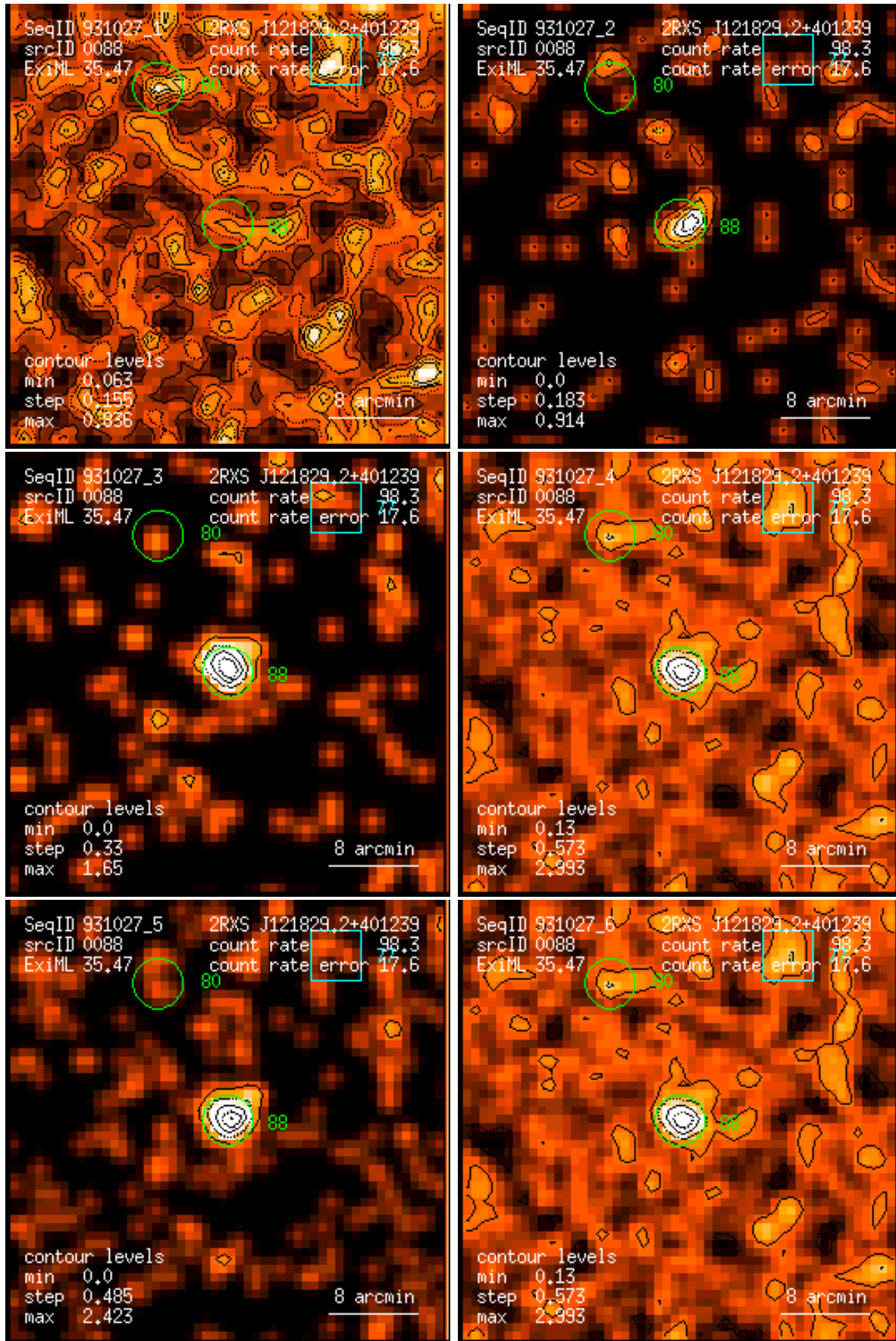
Figure 88: RASS 931027: detection 0088: band rate images, Gaussian filter: (1) PSPC channels 11 – 41, (2) 52 – 90, (3) 91 – 201, (4) 11 – 235, (5) 52 – 201, (6) 11 – 201. Broad band rates in counts/ks. Band rate contour levels in counts/ks/arcmin 2 .
