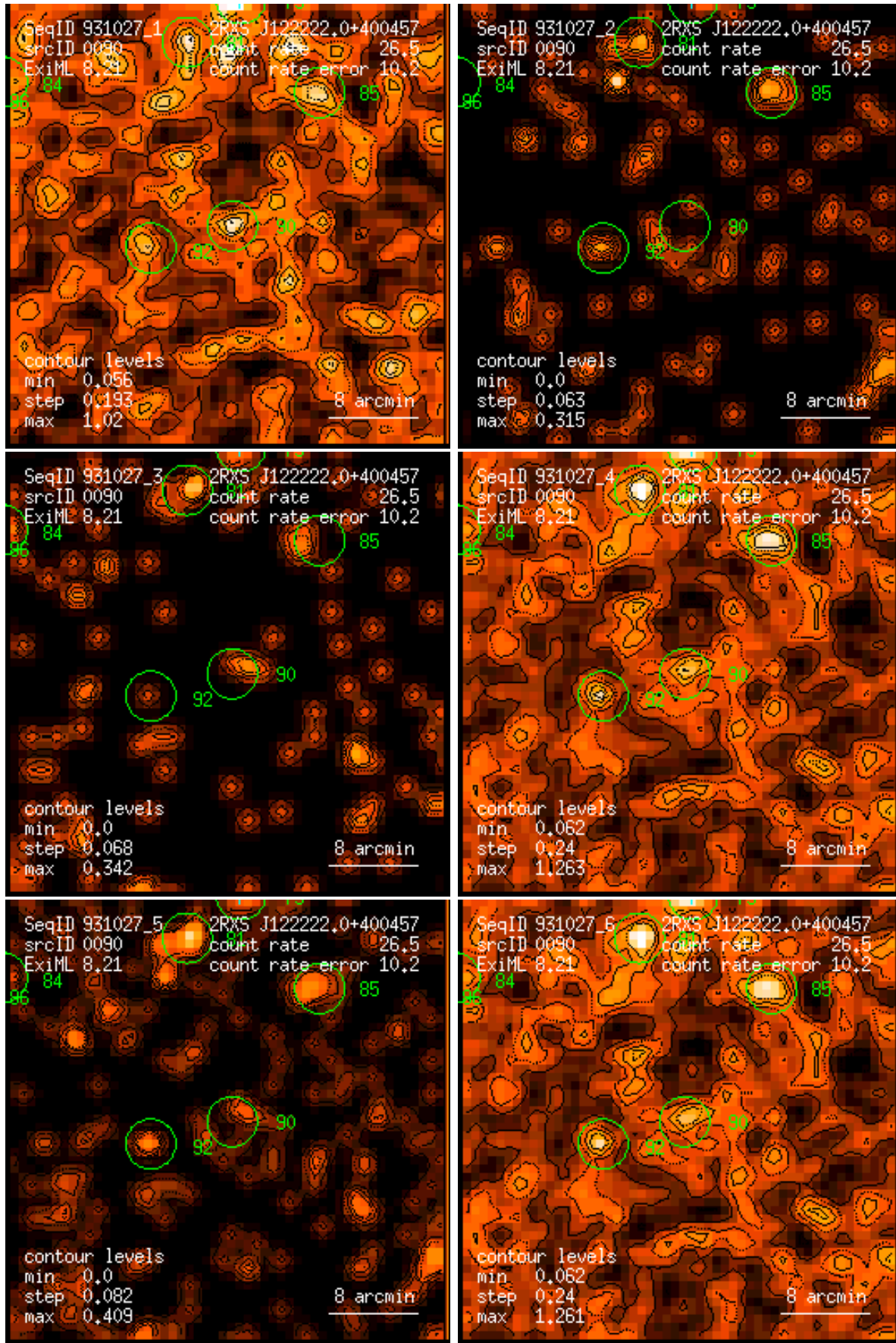
Figure 90: RASS 931027: detection 0090: band rate images, Gaussian filter: (1) PSPC channels 11 – 41, (2) 52 – 90, (3) 91 – 201, (4) 11 – 235, (5) 52 – 201, (6) 11 – 201. Broad band rates in counts/ks. Band rate contour levels in counts/ks/arcmin 2 .
