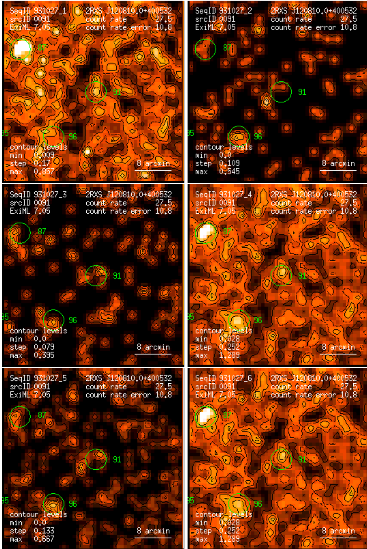
Figure 91: RASS 931027: detection 0091: band rate images, Gaussian filter: (1) PSPC channels 11 – 41, (2) 52 – 90, (3) 91 – 201, (4) 11 – 235, (5) 52 – 201, (6) 11 – 201. Broad band rates in counts/ks. Band rate contour levels in counts/ks/arcmin 2 .
