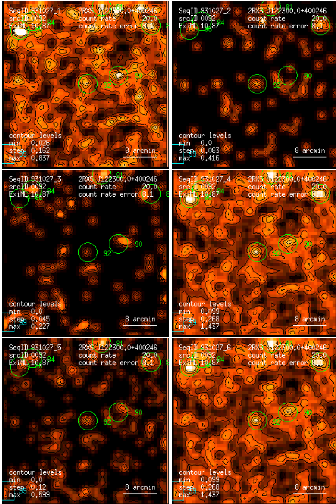
Figure 92: RASS 931027: detection 0092: band rate images, Gaussian filter: (1) PSPC channels 11 – 41, (2) 52 – 90, (3) 91 – 201, (4) 11 – 235, (5) 52 – 201, (6) 11 – 201. Broad band rates in counts/ks. Band rate contour levels in counts/ks/arcmin 2 .
