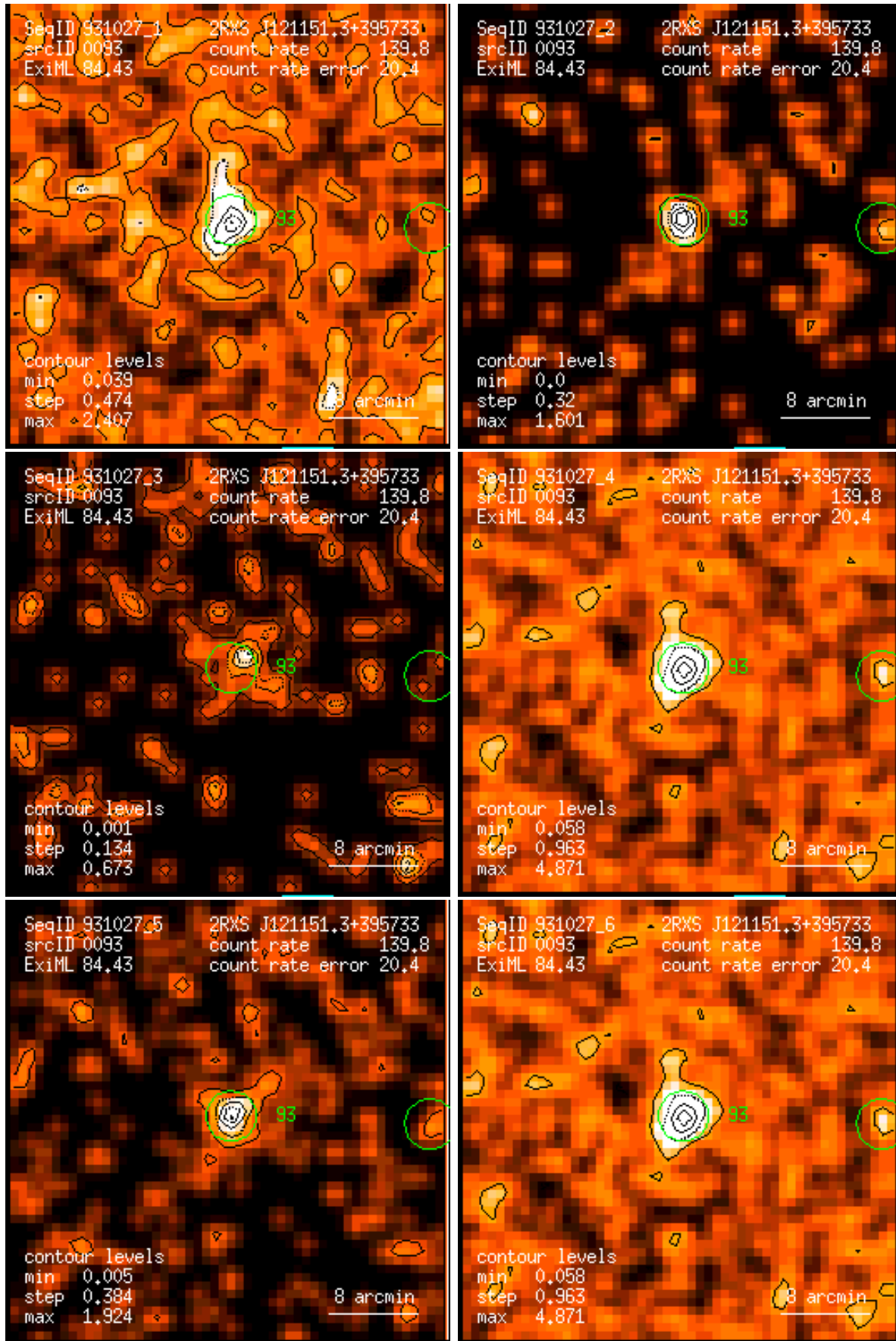
Figure 93: RASS 931027: detection 0093: band rate images, Gaussian filter: (1) PSPC channels 11 – 41, (2) 52 – 90, (3) 91 – 201, (4) 11 – 235, (5) 52 – 201, (6) 11 – 201. Broad band rates in counts/ks. Band rate contour levels in counts/ks/arcmin 2 .
