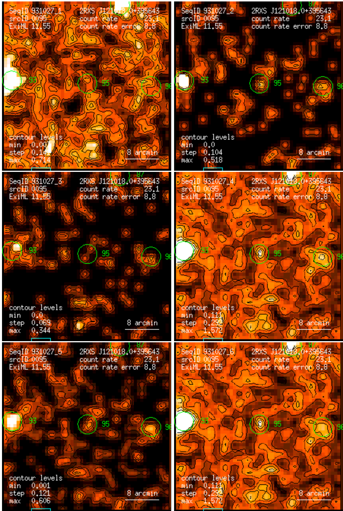
Figure 95: RASS 931027: detection 0095: band rate images, Gaussian filter: (1) PSPC channels 11 – 41, (2) 52 – 90, (3) 91 – 201, (4) 11 – 235, (5) 52 – 201, (6) 11 – 201. Broad band rates in counts/ks. Band rate contour levels in counts/ks/arcmin 2 .
