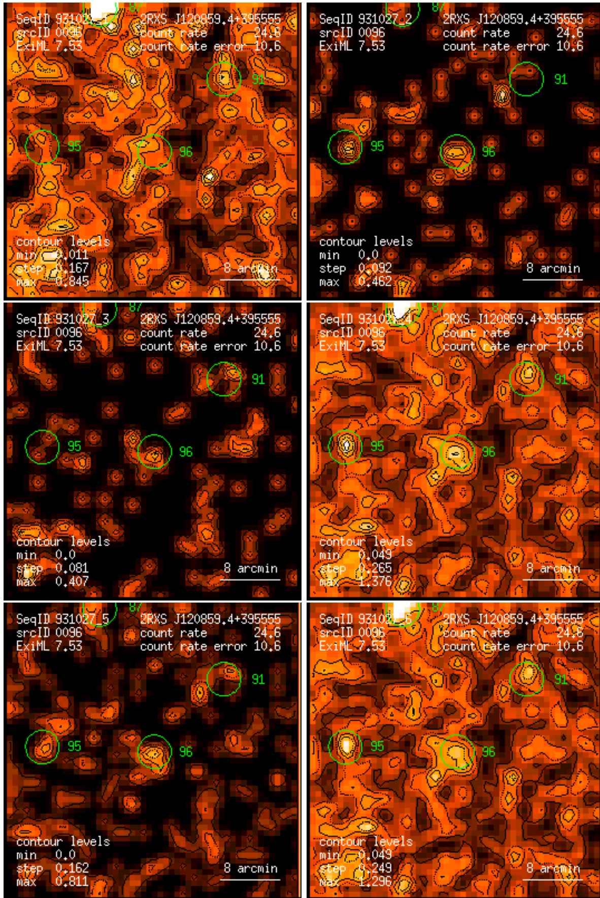
Figure 96: RASS 931027: detection 0096: band rate images, Gaussian filter: (1) PSPC channels 11 – 41, (2) 52 – 90, (3) 91 – 201, (4) 11 – 235, (5) 52 – 201, (6) 11 – 201. Broad band rates in counts/ks. Band rate contour levels in counts/ks/arcmin 2 .
