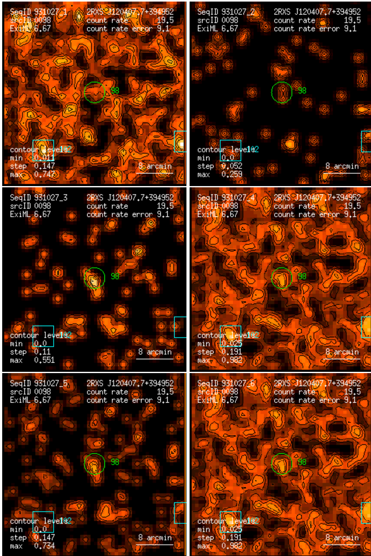
Figure 98: RASS 931027: detection 0098: band rate images, Gaussian filter: (1) PSPC channels 11 – 41, (2) 52 – 90, (3) 91 – 201, (4) 11 – 235, (5) 52 – 201, (6) 11 – 201. Broad band rates in counts/ks. Band rate contour levels in counts/ks/arcmin 2 .
