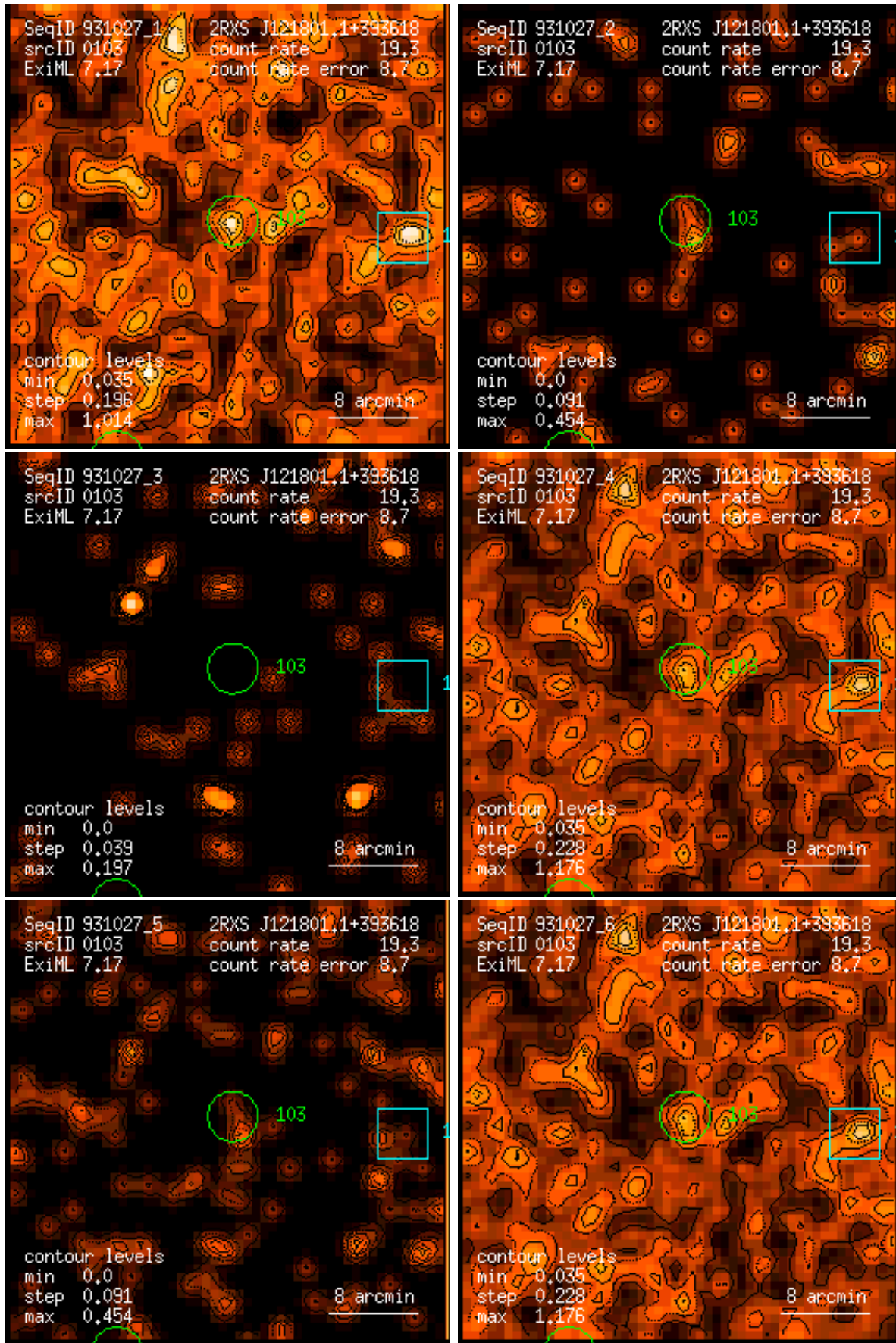
Figure 103: RASS 931027: detection 0103: band rate images, Gaussian filter: (1) PSPC channels 11 – 41, (2) 52 – 90, (3) 91 – 201, (4) 11 – 235, (5) 52 – 201, (6) 11 – 201. Broad band rates in counts/ks. Band rate contour levels in counts/ks/arcmin 2 .
