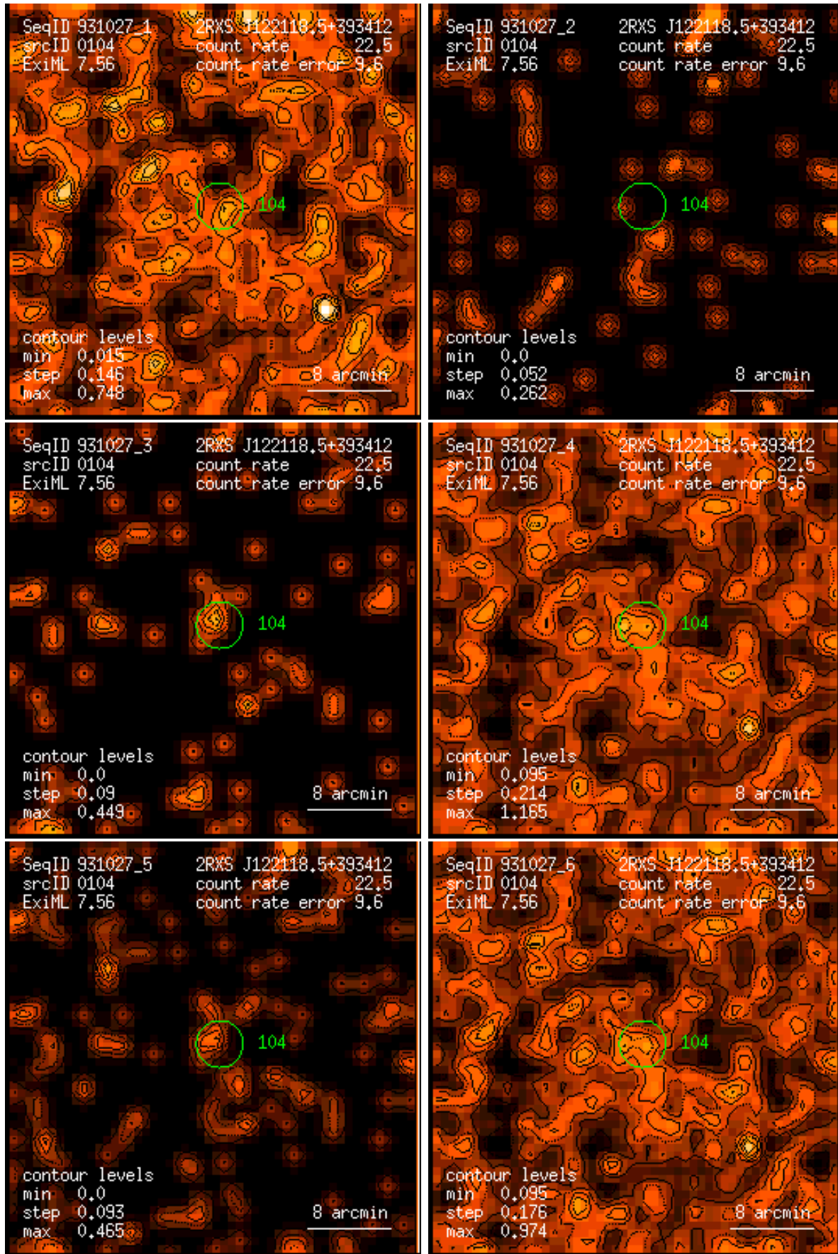
Figure 104: RASS 931027: detection 0104: band rate images, Gaussian filter: (1) PSPC channels 11 – 41, (2) 52 – 90, (3) 91 – 201, (4) 11 – 235, (5) 52 – 201, (6) 11 – 201. Broad band rates in counts/ks. Band rate contour levels in counts/ks/arcmin 2 .
