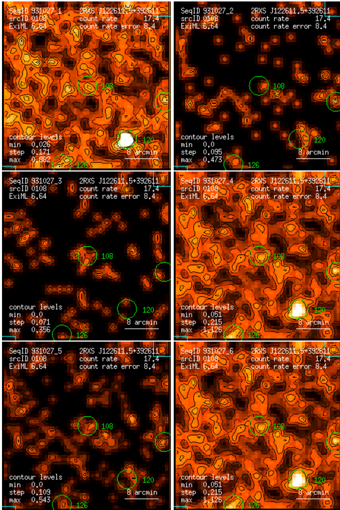
Figure 108: RASS 931027: detection 0108: band rate images, Gaussian filter: (1) PSPC channels 11 – 41, (2) 52 – 90, (3) 91 – 201, (4) 11 – 235, (5) 52 – 201, (6) 11 – 201. Broad band rates in counts/ks. Band rate contour levels in counts/ks/arcmin 2 .
