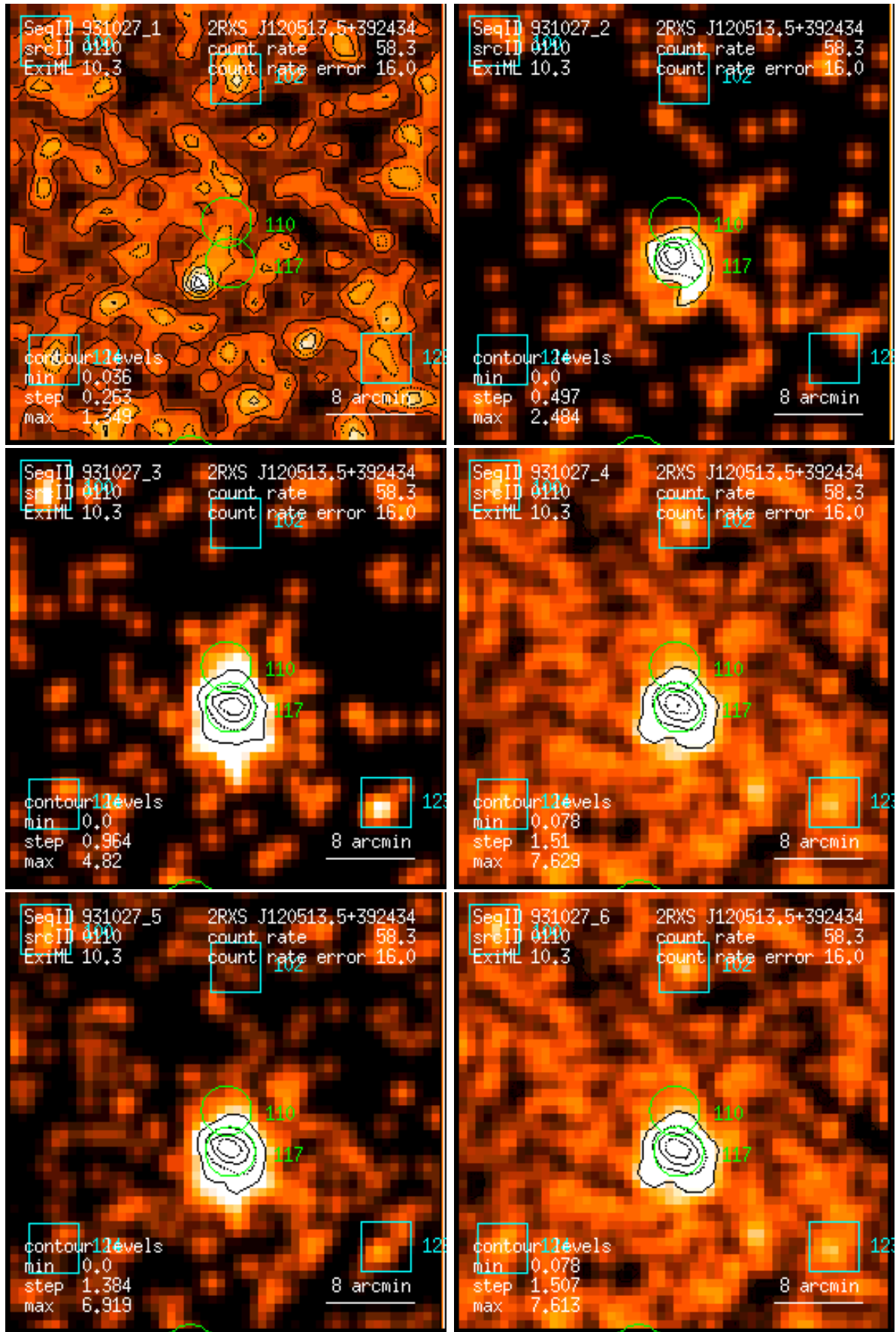
Figure 110: RASS 931027: detection 0110: band rate images, Gaussian filter: (1) PSPC channels 11 – 41, (2) 52 – 90, (3) 91 – 201, (4) 11 – 235, (5) 52 – 201, (6) 11 – 201. Broad band rates in counts/ks. Band rate contour levels in counts/ks/arcmin 2 .
