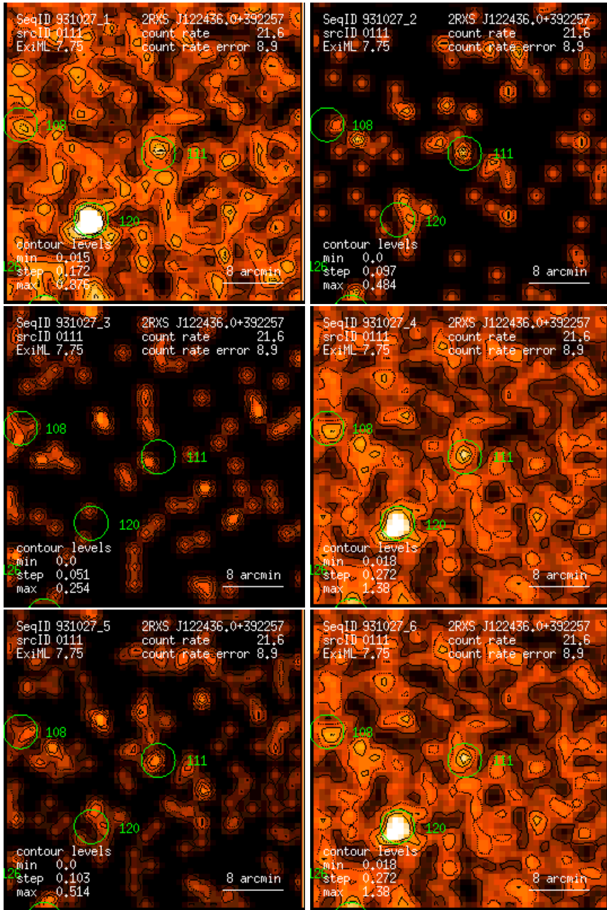
Figure 111: RASS 931027: detection 0111: band rate images, Gaussian filter: (1) PSPC channels 11 – 41, (2) 52 – 90, (3) 91 – 201, (4) 11 – 235, (5) 52 – 201, (6) 11 – 201. Broad band rates in counts/ks. Band rate contour levels in counts/ks/arcmin 2 .
