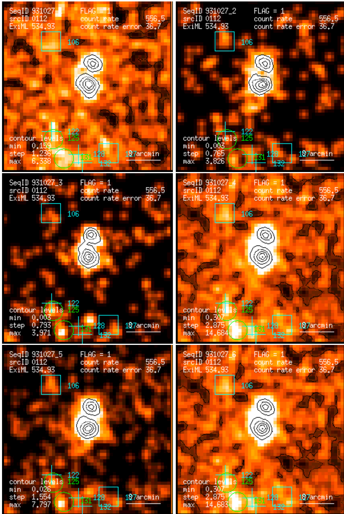
Figure 112: RASS 931027: detection 0112: band rate images, Gaussian filter: (1) PSPC channels 11 – 41, (2) 52 – 90, (3) 91 – 201, (4) 11 – 235, (5) 52 – 201, (6) 11 – 201. Broad band rates in counts/ks. Band rate contour levels in counts/ks/arcmin 2 .
