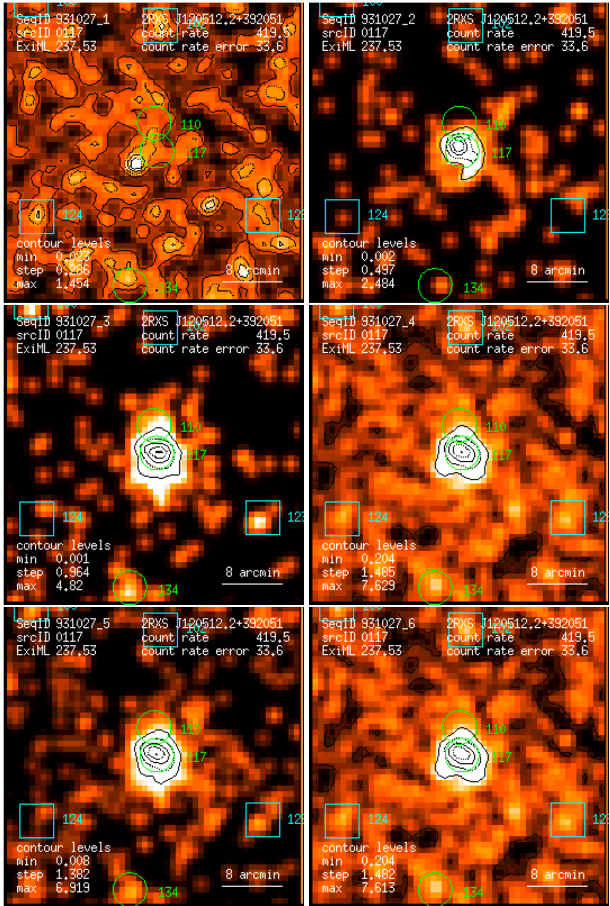
Figure 117: RASS 931027: detection 0117: band rate images, Gaussian filter: (1) PSPC channels 11 – 41, (2) 52 – 90, (3) 91 – 201, (4) 11 – 235, (5) 52 – 201, (6) 11 – 201. Broad band rates in counts/ks. Band rate contour levels in counts/ks/arcmin 2 .
