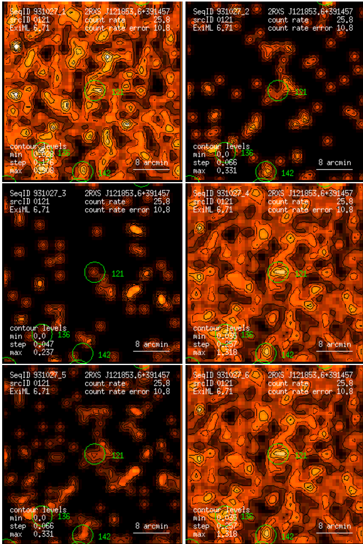
Figure 121: RASS 931027: detection 0121: band rate images, Gaussian filter: (1) PSPC channels 11 – 41, (2) 52 – 90, (3) 91 – 201, (4) 11 – 235, (5) 52 – 201, (6) 11 – 201. Broad band rates in counts/ks. Band rate contour levels in counts/ks/arcmin 2 .
