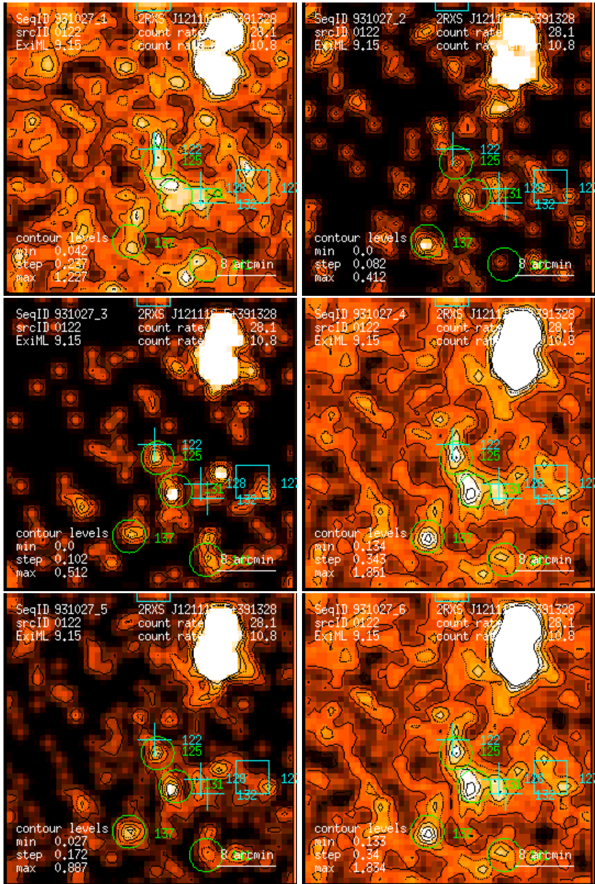
Figure 122: RASS 931027: detection 0122: band rate images, Gaussian filter: (1) PSPC channels 11 – 41, (2) 52 – 90, (3) 91 – 201, (4) 11 – 235, (5) 52 – 201, (6) 11 – 201. Broad band rates in counts/ks. Band rate contour levels in counts/ks/arcmin 2 .
