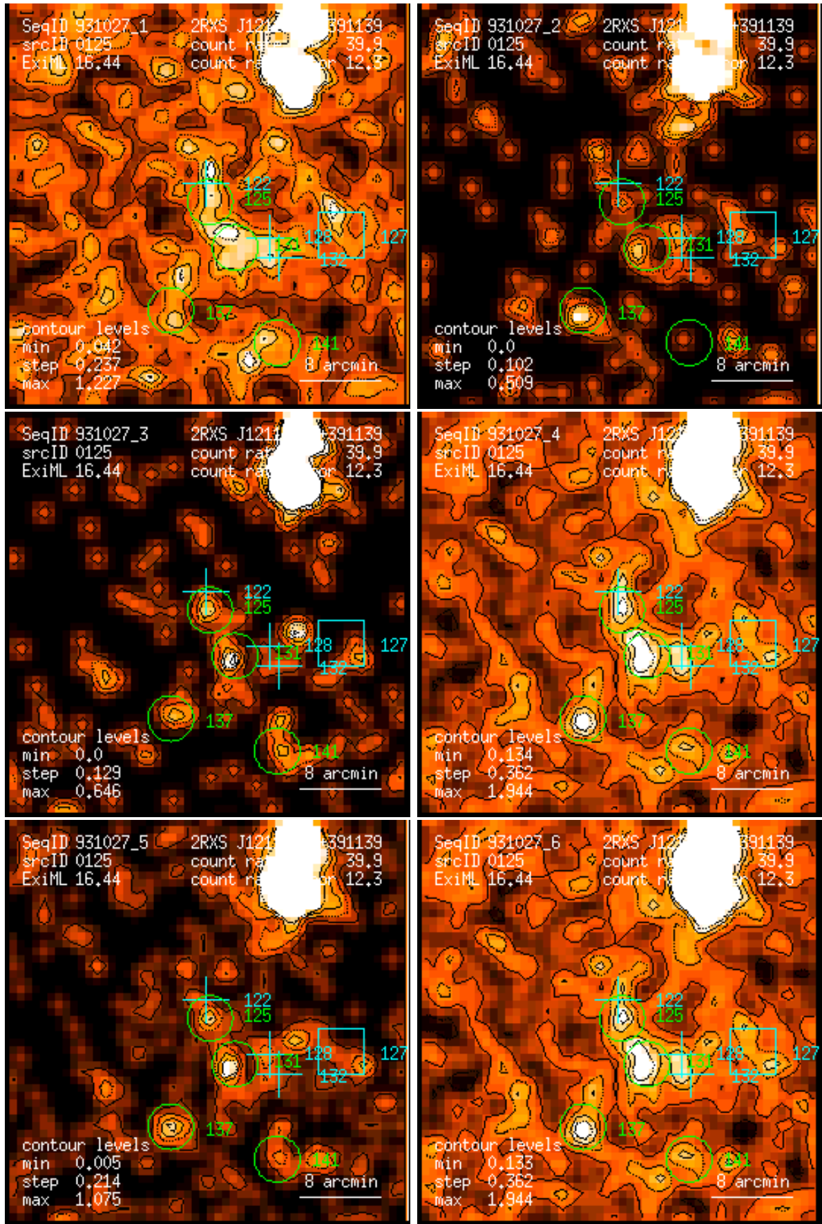
Figure 125: RASS 931027: detection 0125: band rate images, Gaussian filter: (1) PSPC channels 11 – 41, (2) 52 – 90, (3) 91 – 201, (4) 11 – 235, (5) 52 – 201, (6) 11 – 201. Broad band rates in counts/ks. Band rate contour levels in counts/ks/arcmin 2 .
