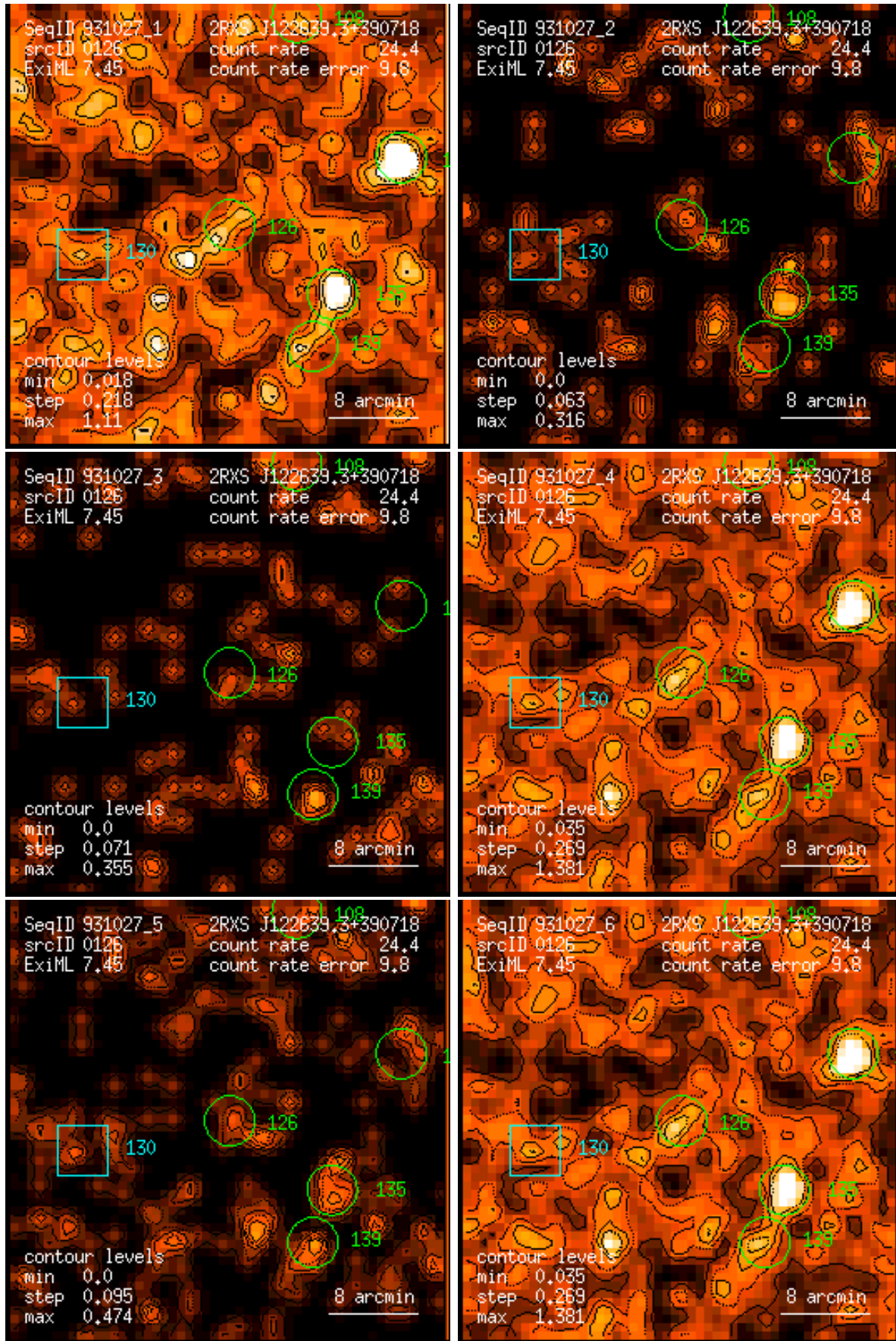
Figure 126: RASS 931027: detection 0126: band rate images, Gaussian filter: (1) PSPC channels 11 – 41, (2) 52 – 90, (3) 91 – 201, (4) 11 – 235, (5) 52 – 201, (6) 11 – 201. Broad band rates in counts/ks. Band rate contour levels in counts/ks/arcmin 2 .
