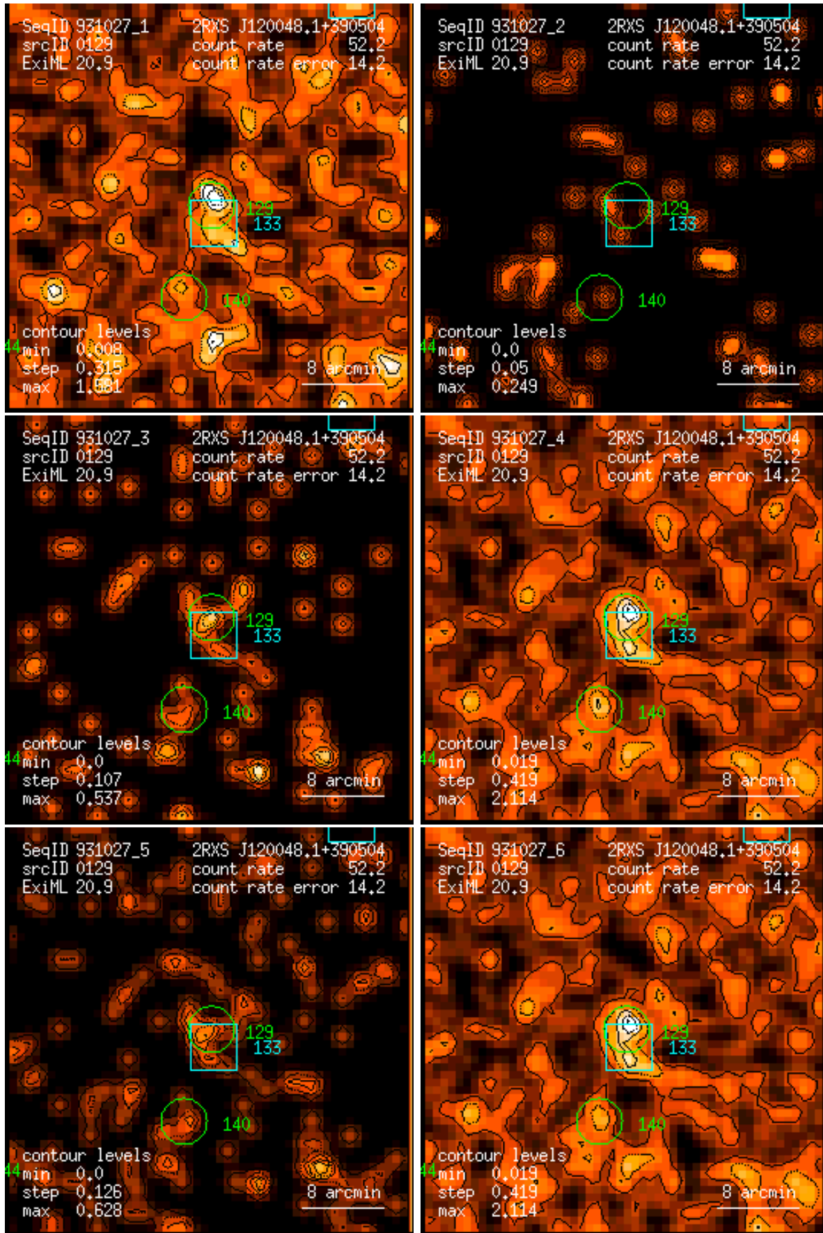
Figure 129: RASS 931027: detection 0129: band rate images, Gaussian filter: (1) PSPC channels 11 – 41, (2) 52 – 90, (3) 91 – 201, (4) 11 – 235, (5) 52 – 201, (6) 11 – 201. Broad band rates in counts/ks. Band rate contour levels in counts/ks/arcmin 2 .
