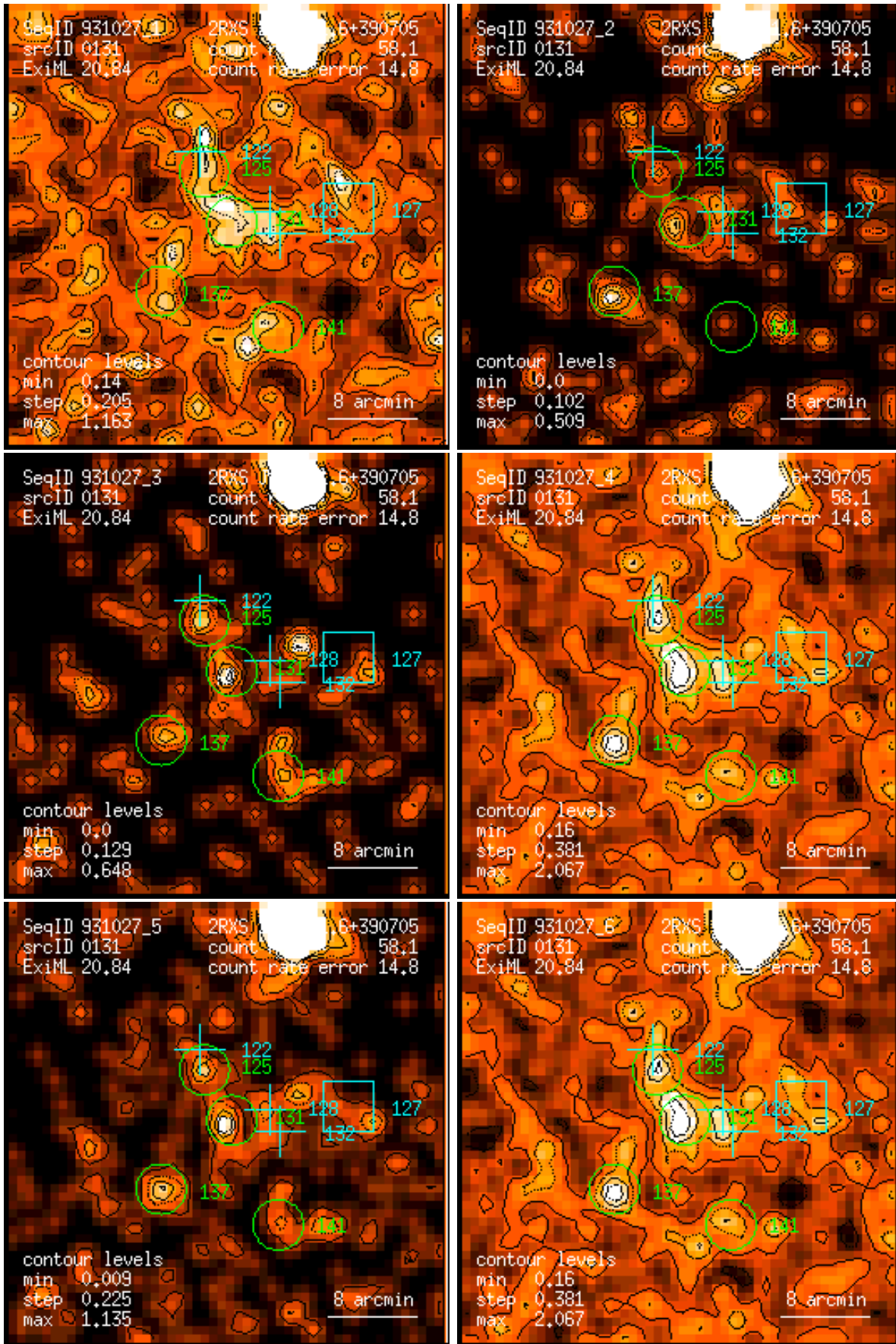
Figure 131: RASS 931027: detection 0131: band rate images, Gaussian filter: (1) PSPC channels 11 – 41, (2) 52 – 90, (3) 91 – 201, (4) 11 – 235, (5) 52 – 201, (6) 11 – 201. Broad band rates in counts/ks. Band rate contour levels in counts/ks/arcmin 2 .
