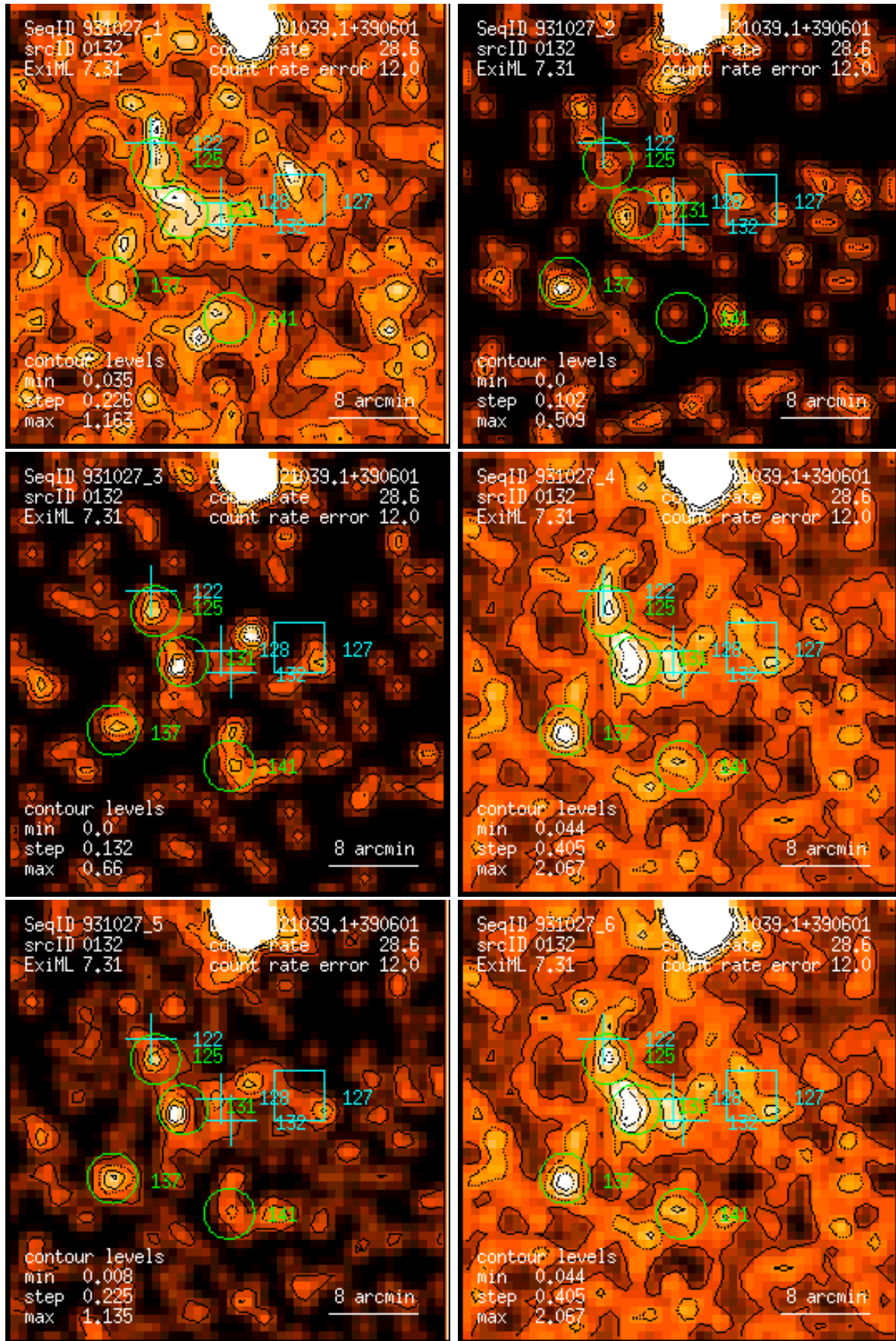
Figure 132: RASS 931027: detection 0132: band rate images, Gaussian filter: (1) PSPC channels 11 – 41, (2) 52 – 90, (3) 91 – 201, (4) 11 – 235, (5) 52 – 201, (6) 11 – 201. Broad band rates in counts/ks. Band rate contour levels in counts/ks/arcmin 2 .
