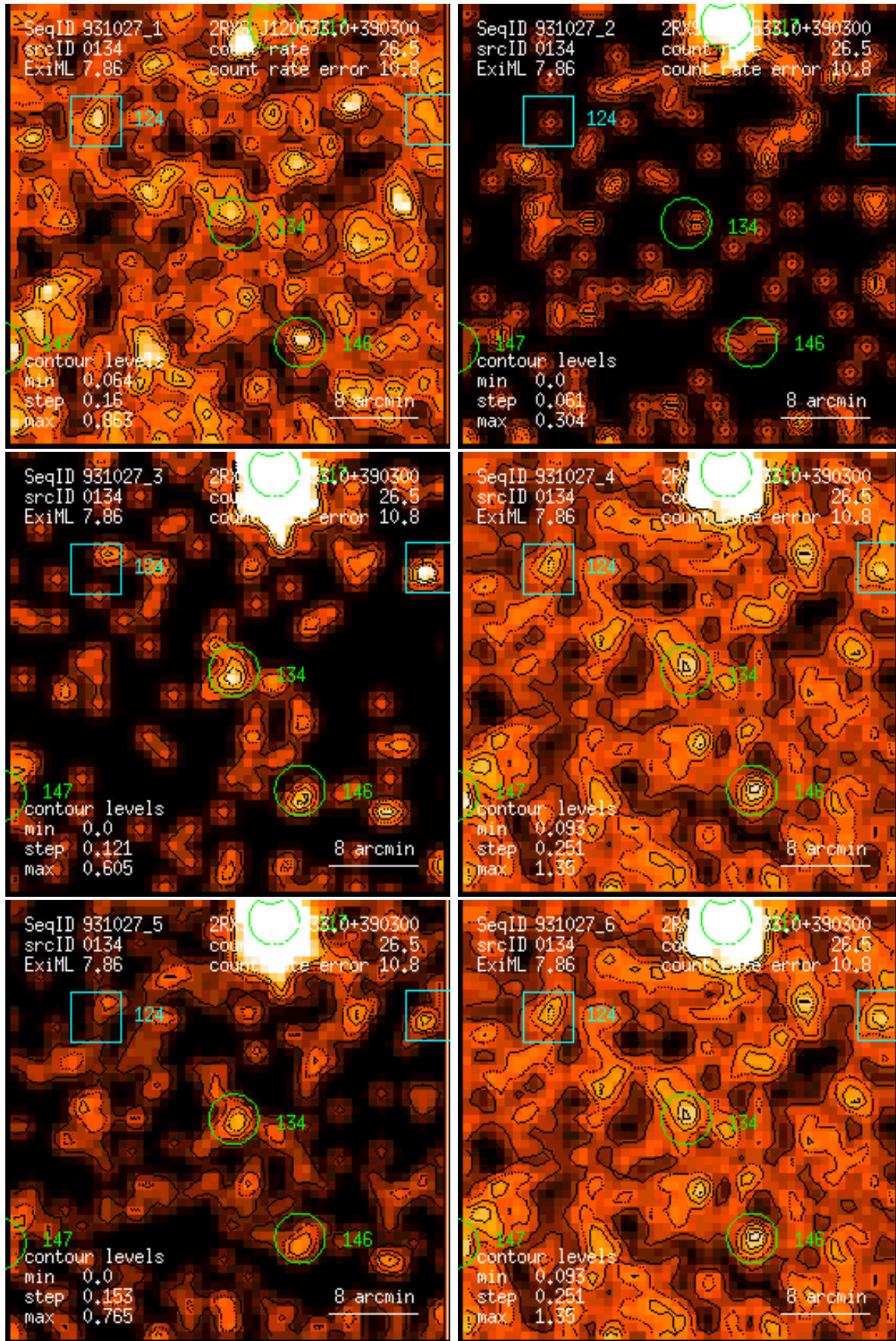
Figure 134: RASS 931027: detection 0134: band rate images, Gaussian filter: (1) PSPC channels 11 – 41, (2) 52 – 90, (3) 91 – 201, (4) 11 – 235, (5) 52 – 201, (6) 11 – 201. Broad band rates in counts/ks. Band rate contour levels in counts/ks/arcmin 2 .
