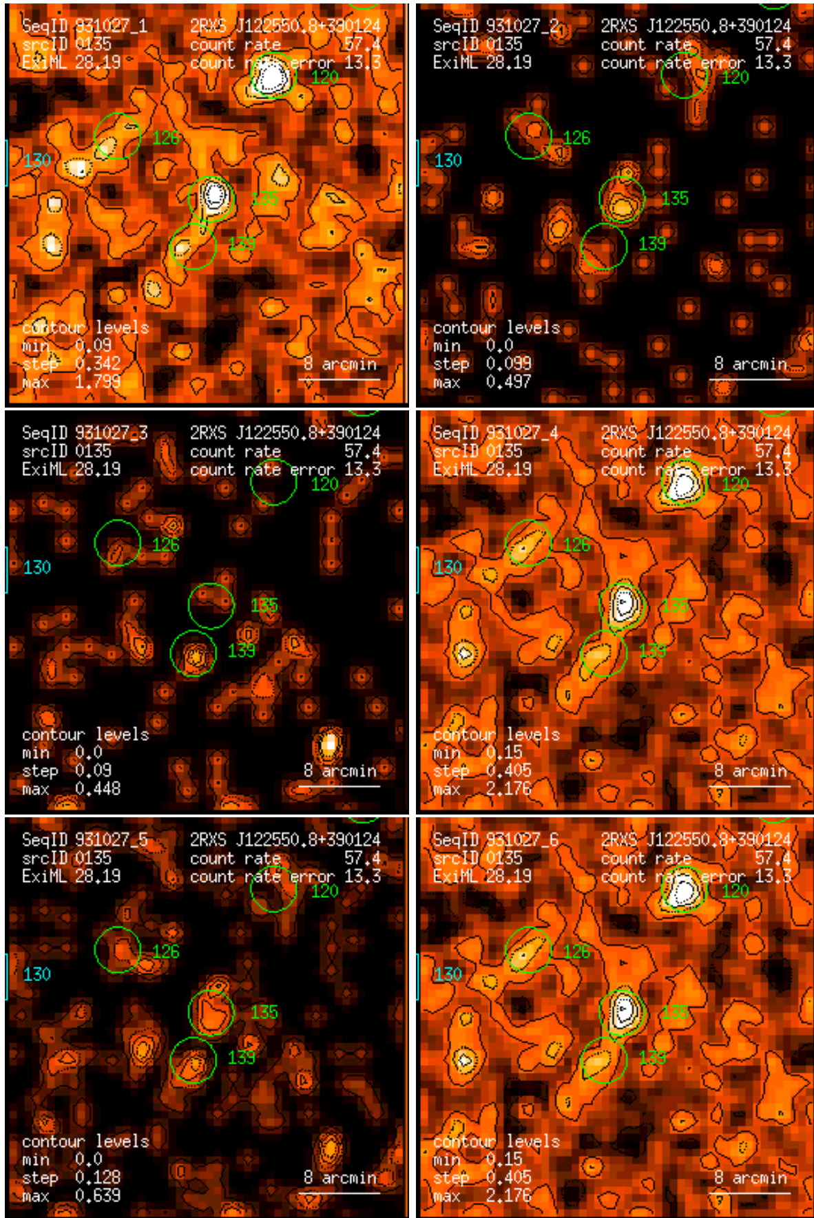
Figure 135: RASS 931027: detection 0135: band rate images, Gaussian filter: (1) PSPC channels 11 – 41, (2) 52 – 90, (3) 91 – 201, (4) 11 – 235, (5) 52 – 201, (6) 11 – 201. Broad band rates in counts/ks. Band rate contour levels in counts/ks/arcmin 2 .
