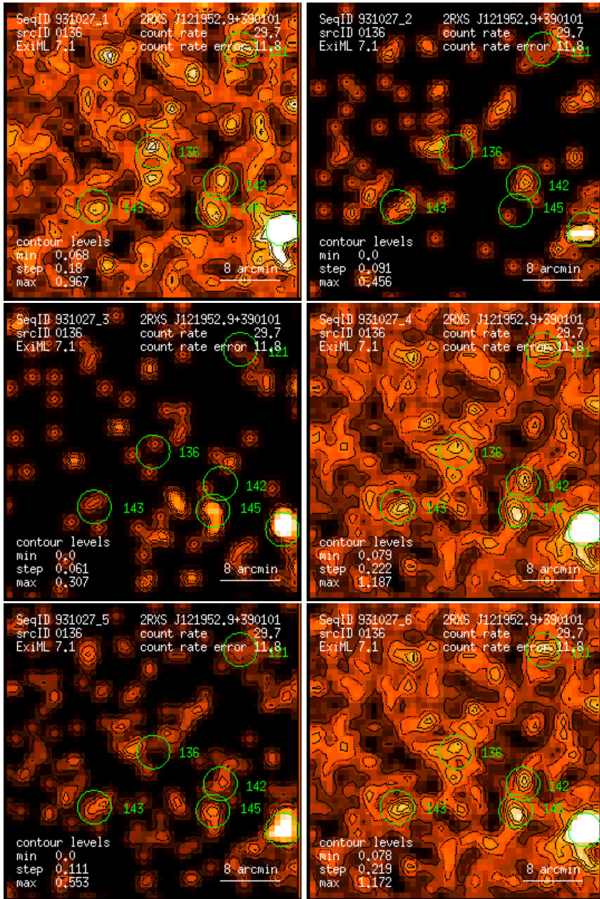
Figure 136: RASS 931027: detection 0136: band rate images, Gaussian filter: (1) PSPC channels 11 – 41, (2) 52 – 90, (3) 91 – 201, (4) 11 – 235, (5) 52 – 201, (6) 11 – 201. Broad band rates in counts/ks. Band rate contour levels in counts/ks/arcmin 2 .
