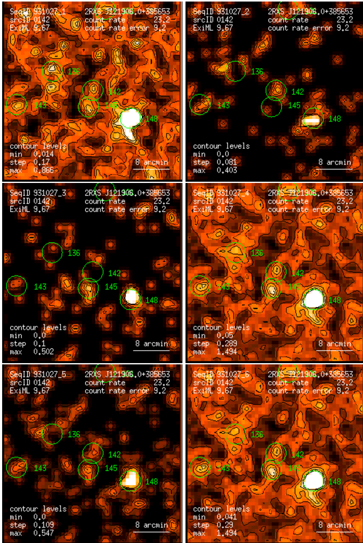
Figure 142: RASS 931027: detection 0142: band rate images, Gaussian filter: (1) PSPC channels 11 – 41, (2) 52 – 90, (3) 91 – 201, (4) 11 – 235, (5) 52 – 201, (6) 11 – 201. Broad band rates in counts/ks. Band rate contour levels in counts/ks/arcmin 2 .
