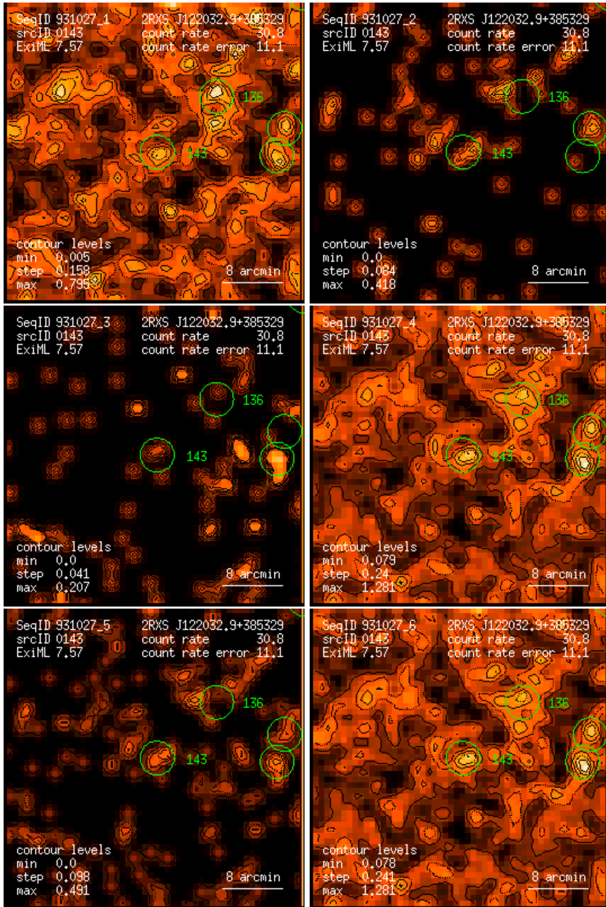
Figure 143: RASS 931027: detection 0143: band rate images, Gaussian filter: (1) PSPC channels 11 – 41, (2) 52 – 90, (3) 91 – 201, (4) 11 – 235, (5) 52 – 201, (6) 11 – 201. Broad band rates in counts/ks. Band rate contour levels in counts/ks/arcmin 2 .
