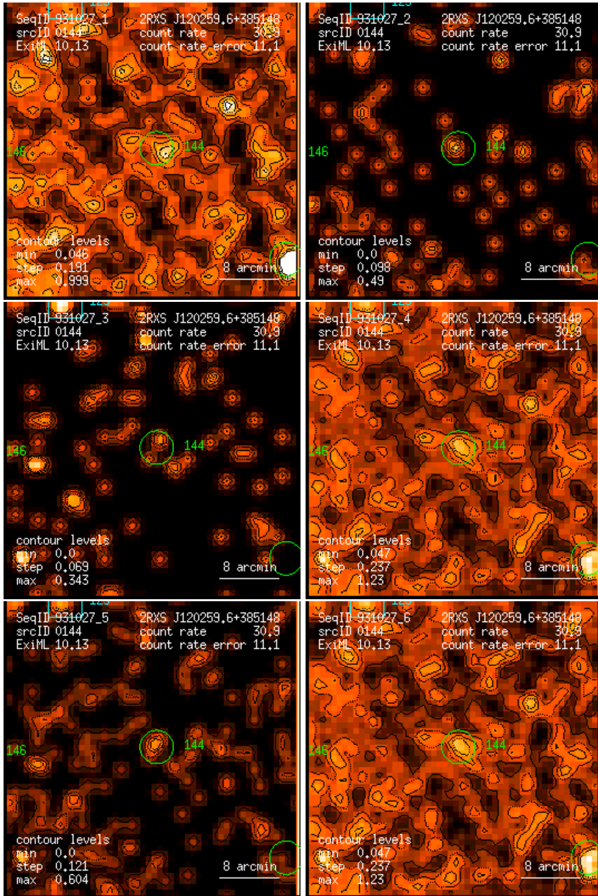
Figure 144: RASS 931027: detection 0144: band rate images, Gaussian filter: (1) PSPC channels 11 – 41, (2) 52 – 90, (3) 91 – 201, (4) 11 – 235, (5) 52 – 201, (6) 11 – 201. Broad band rates in counts/ks. Band rate contour levels in counts/ks/arcmin 2 .
