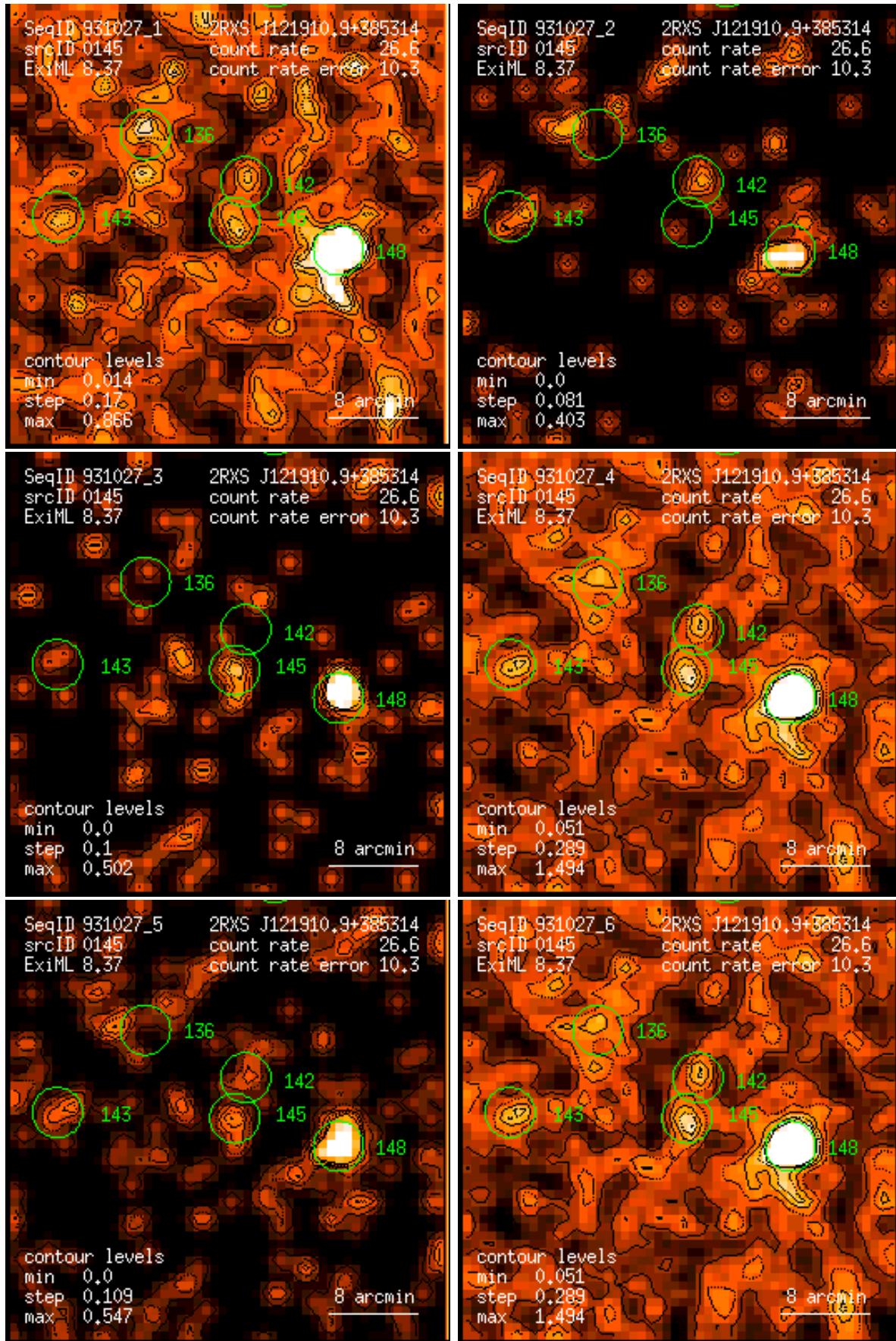
Figure 145: RASS 931027: detection 0145: band rate images, Gaussian filter: (1) PSPC channels 11 – 41, (2) 52 – 90, (3) 91 – 201, (4) 11 – 235, (5) 52 – 201, (6) 11 – 201. Broad band rates in counts/ks. Band rate contour levels in counts/ks/arcmin 2 .
