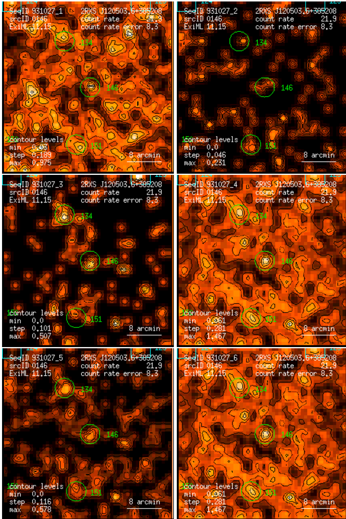
Figure 146: RASS 931027: detection 0146: band rate images, Gaussian filter: (1) PSPC channels 11 – 41, (2) 52 – 90, (3) 91 – 201, (4) 11 – 235, (5) 52 – 201, (6) 11 – 201. Broad band rates in counts/ks. Band rate contour levels in counts/ks/arcmin 2 .
