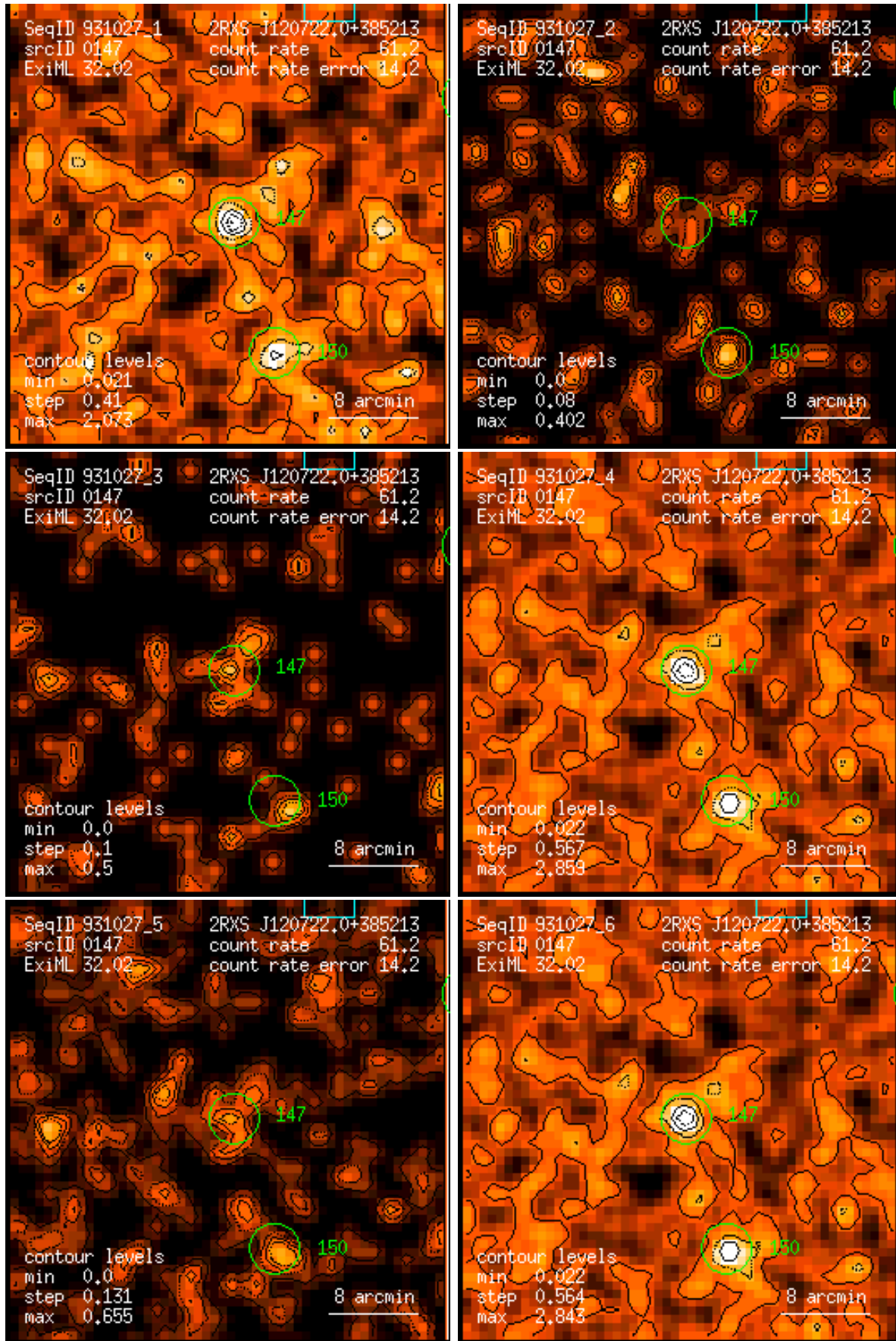
Figure 147: RASS 931027: detection 0147: band rate images, Gaussian filter: (1) PSPC channels 11 – 41, (2) 52 – 90, (3) 91 – 201, (4) 11 – 235, (5) 52 – 201, (6) 11 – 201. Broad band rates in counts/ks. Band rate contour levels in counts/ks/arcmin 2 .
