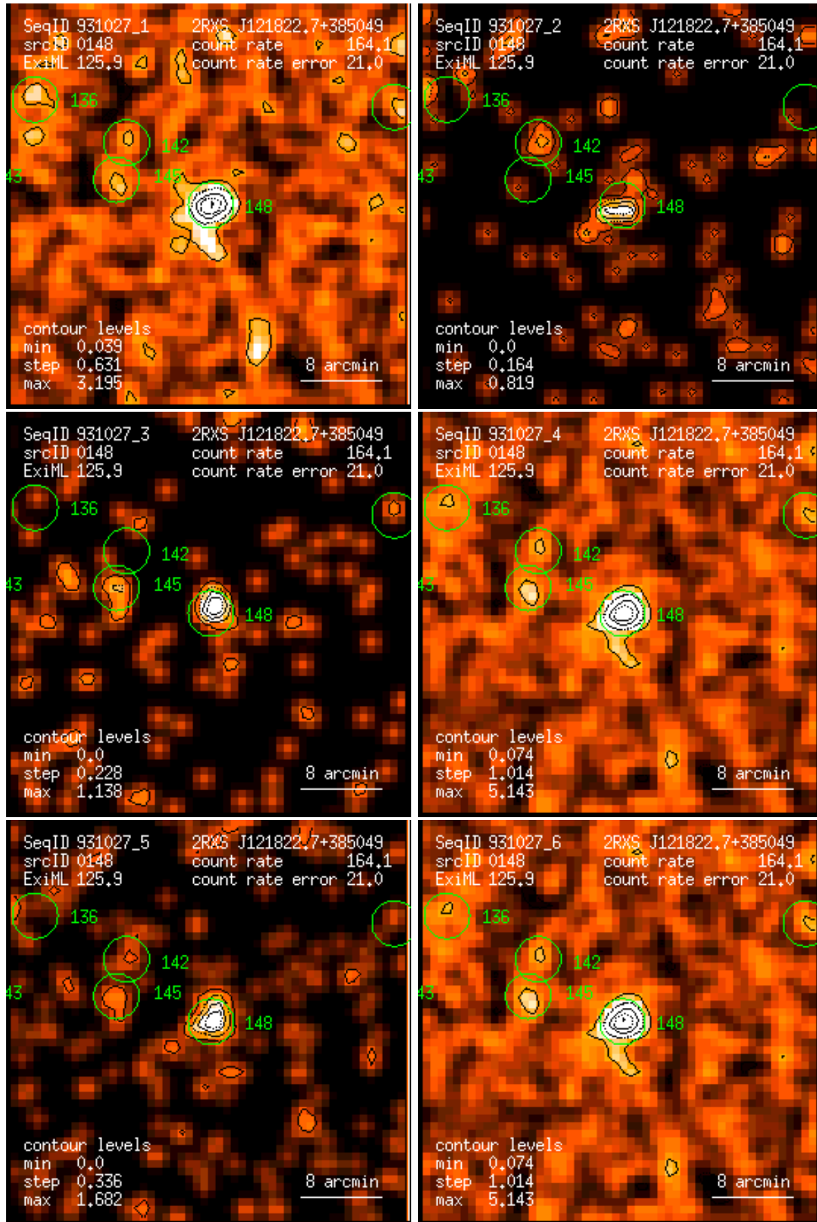
Figure 148: RASS 931027: detection 0148: band rate images, Gaussian filter: (1) PSPC channels 11 – 41, (2) 52 – 90, (3) 91 – 201, (4) 11 – 235, (5) 52 – 201, (6) 11 – 201. Broad band rates in counts/ks. Band rate contour levels in counts/ks/arcmin 2 .
