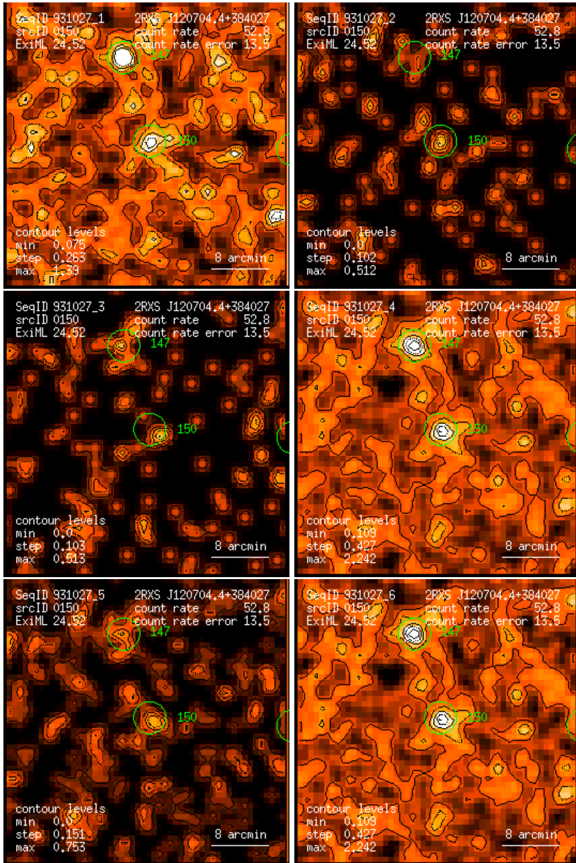
Figure 150: RASS 931027: detection 0150: band rate images, Gaussian filter: (1) PSPC channels 11 – 41, (2) 52 – 90, (3) 91 – 201, (4) 11 – 235, (5) 52 – 201, (6) 11 – 201. Broad band rates in counts/ks. Band rate contour levels in counts/ks/arcmin 2 .
