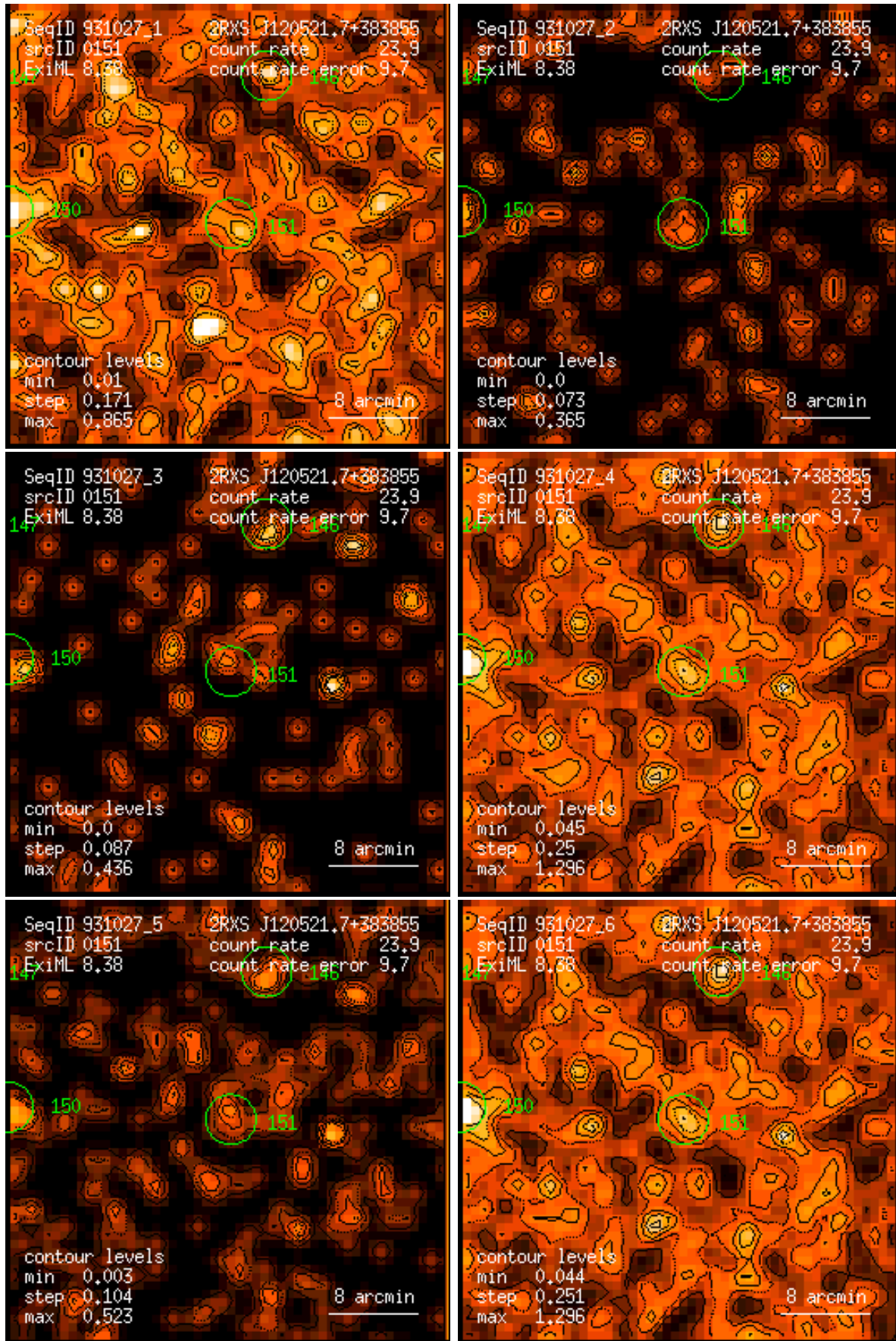
Figure 151: RASS 931027: detection 0151: band rate images, Gaussian filter: (1) PSPC channels 11 – 41, (2) 52 – 90, (3) 91 – 201, (4) 11 – 235, (5) 52 – 201, (6) 11 – 201. Broad band rates in counts/ks. Band rate contour levels in counts/ks/arcmin 2 .
