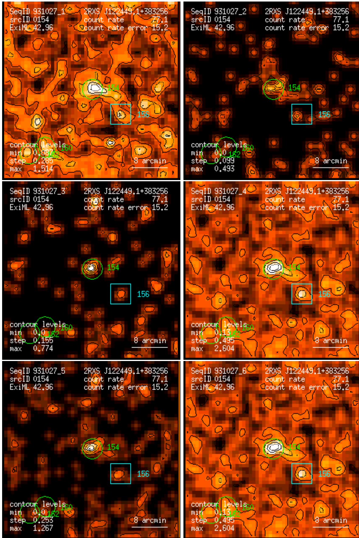
Figure 154: RASS 931027: detection 0154: band rate images, Gaussian filter: (1) PSPC channels 11 – 41, (2) 52 – 90, (3) 91 – 201, (4) 11 – 235, (5) 52 – 201, (6) 11 – 201. Broad band rates in counts/ks. Band rate contour levels in counts/ks/arcmin 2 .
