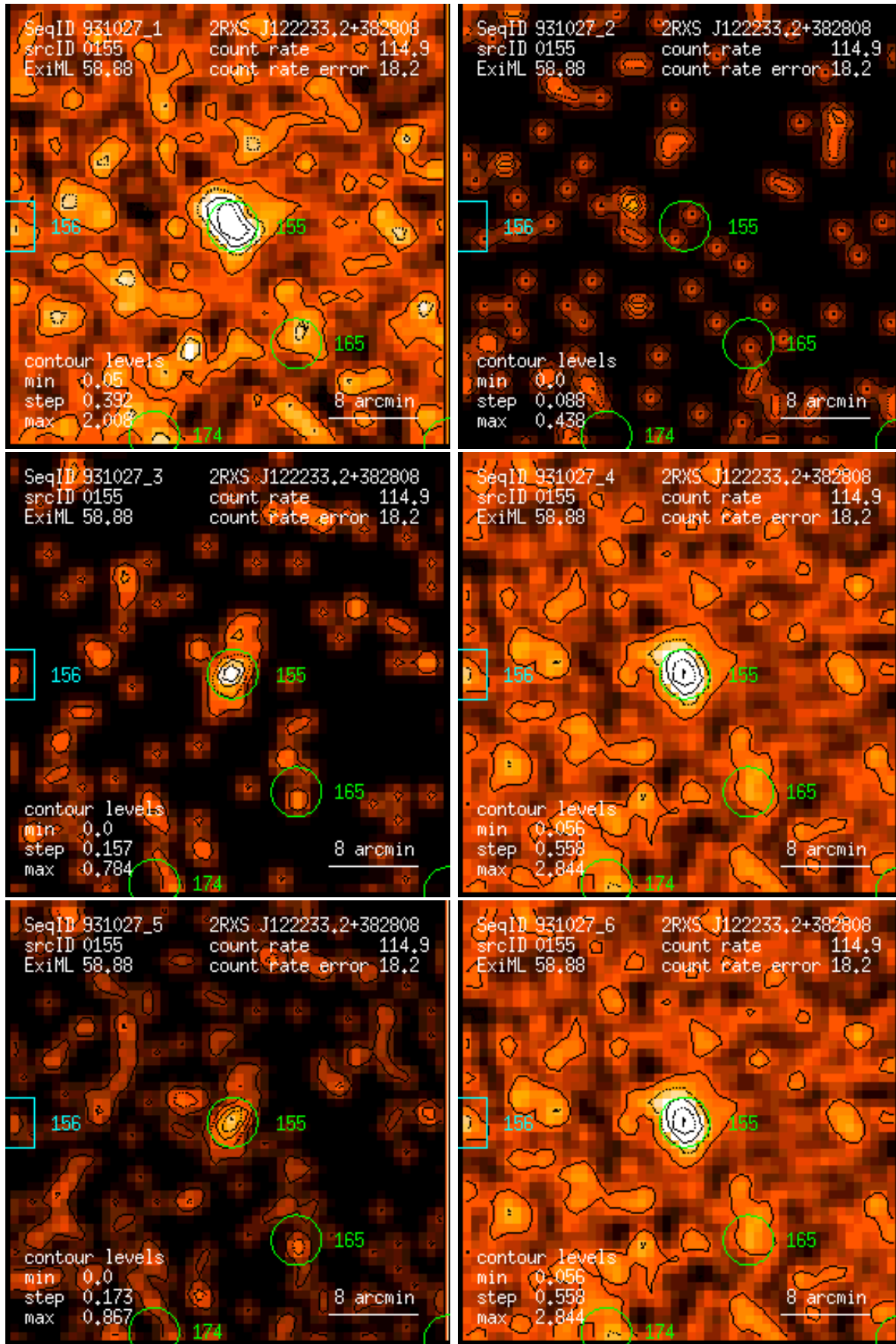
Figure 155: RASS 931027: detection 0155: band rate images, Gaussian filter: (1) PSPC channels 11 – 41, (2) 52 – 90, (3) 91 – 201, (4) 11 – 235, (5) 52 – 201, (6) 11 – 201. Broad band rates in counts/ks. Band rate contour levels in counts/ks/arcmin 2 .
