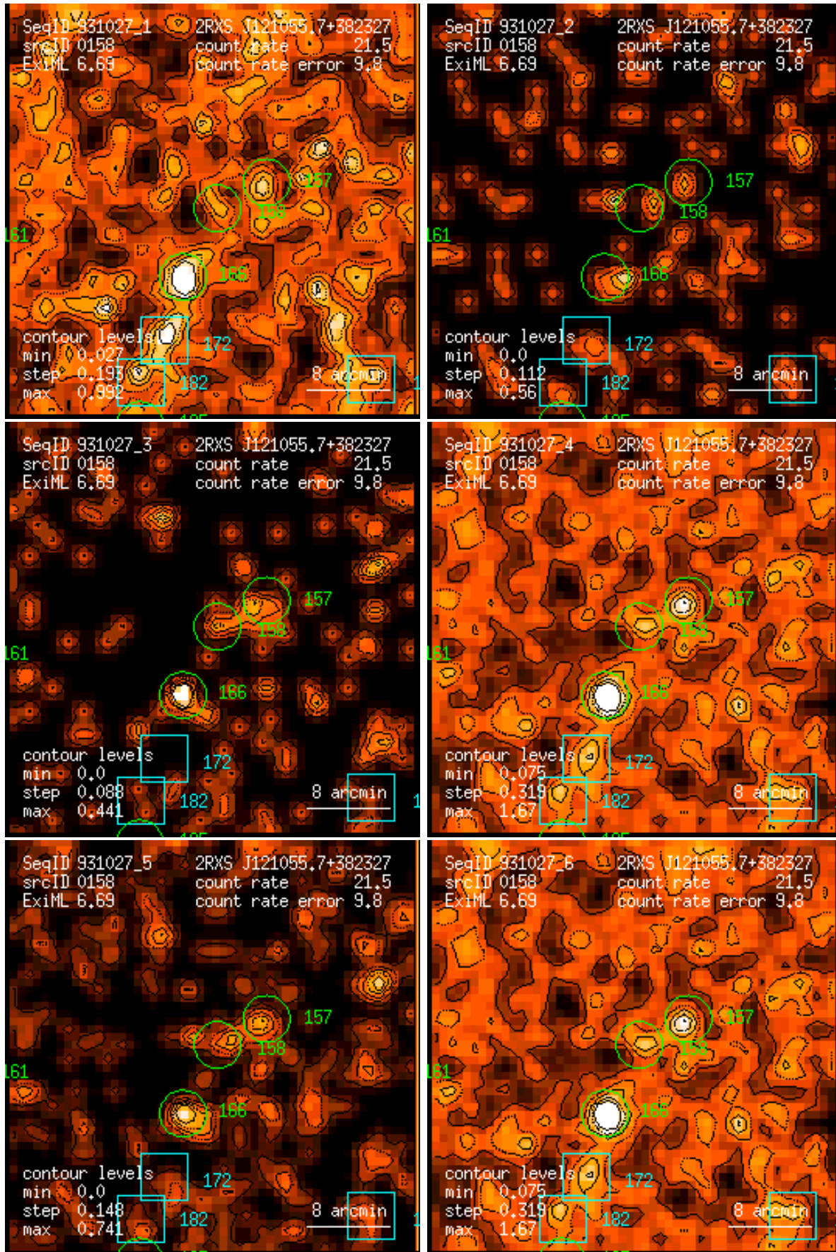
Figure 158: RASS 931027: detection 0158: band rate images, Gaussian filter: (1) PSPC channels 11 – 41, (2) 52 – 90, (3) 91 – 201, (4) 11 – 235, (5) 52 – 201, (6) 11 – 201. Broad band rates in counts/ks. Band rate contour levels in counts/ks/arcmin 2 .
