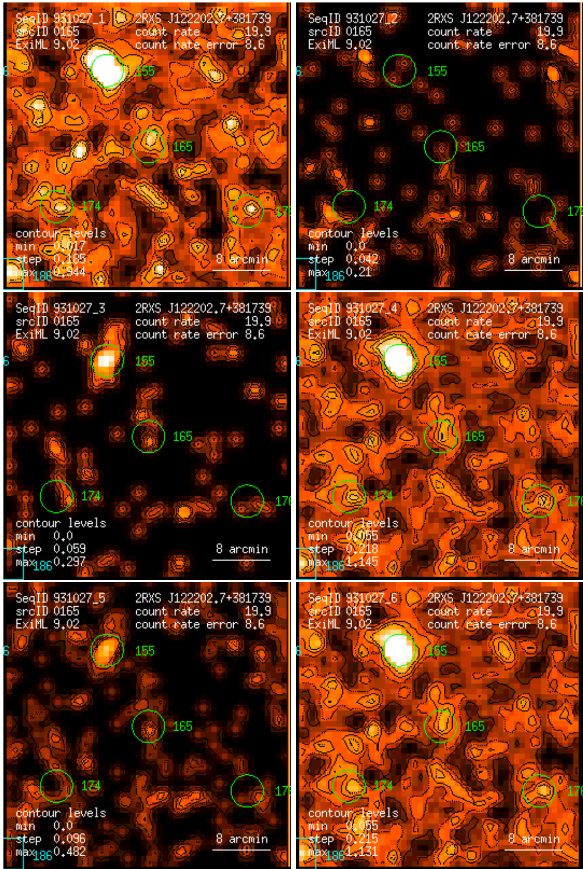
Figure 165: RASS 931027: detection 0165: band rate images, Gaussian filter: (1) PSPC channels 11 – 41, (2) 52 – 90, (3) 91 – 201, (4) 11 – 235, (5) 52 – 201, (6) 11 – 201. Broad band rates in counts/ks. Band rate contour levels in counts/ks/arcmin 2 .
