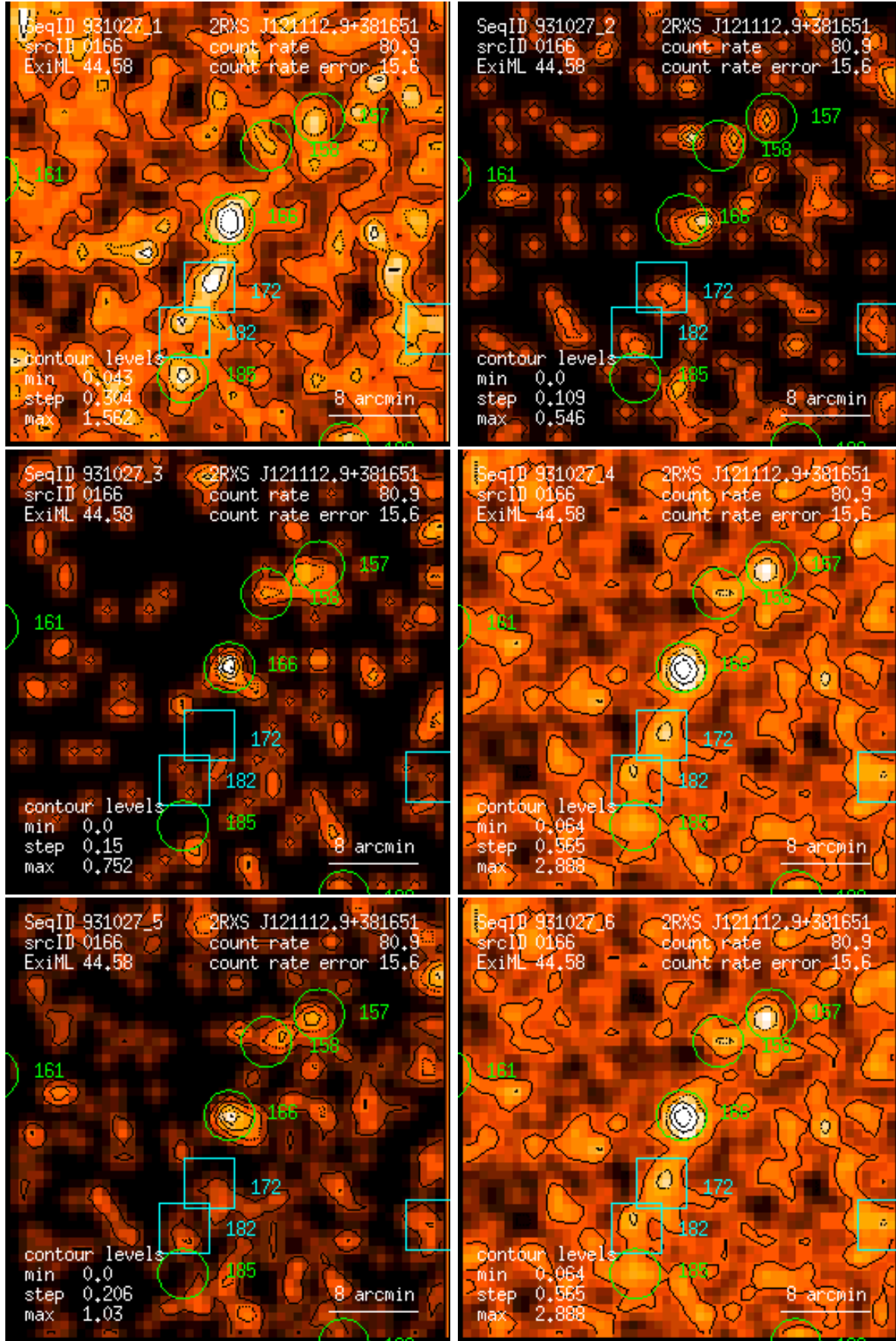
Figure 166: RASS 931027: detection 0166: band rate images, Gaussian filter: (1) PSPC channels 11 – 41, (2) 52 – 90, (3) 91 – 201, (4) 11 – 235, (5) 52 – 201, (6) 11 – 201. Broad band rates in counts/ks. Band rate contour levels in counts/ks/arcmin 2 .
