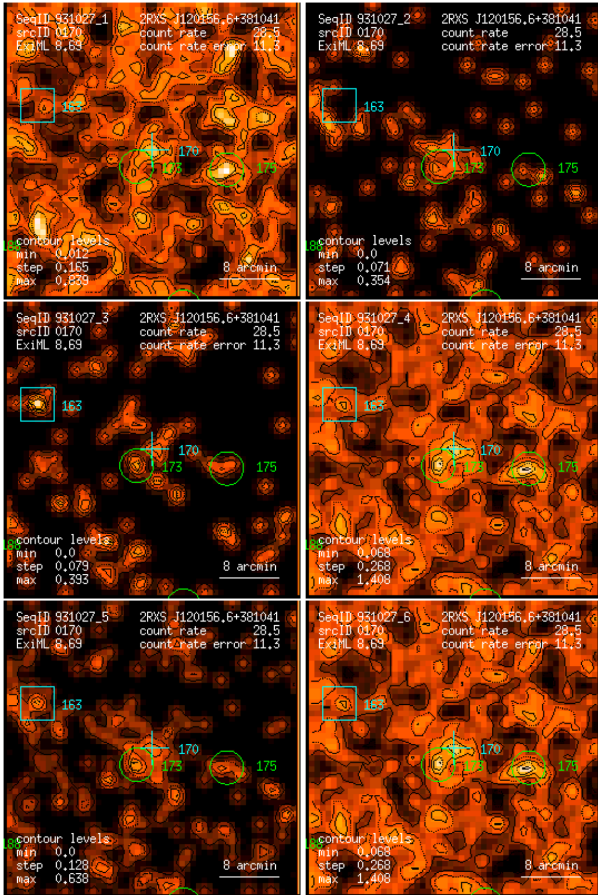
Figure 170: RASS 931027: detection 0170: band rate images, Gaussian filter: (1) PSPC channels 11 – 41, (2) 52 – 90, (3) 91 – 201, (4) 11 – 235, (5) 52 – 201, (6) 11 – 201. Broad band rates in counts/ks. Band rate contour levels in counts/ks/arcmin 2 .
