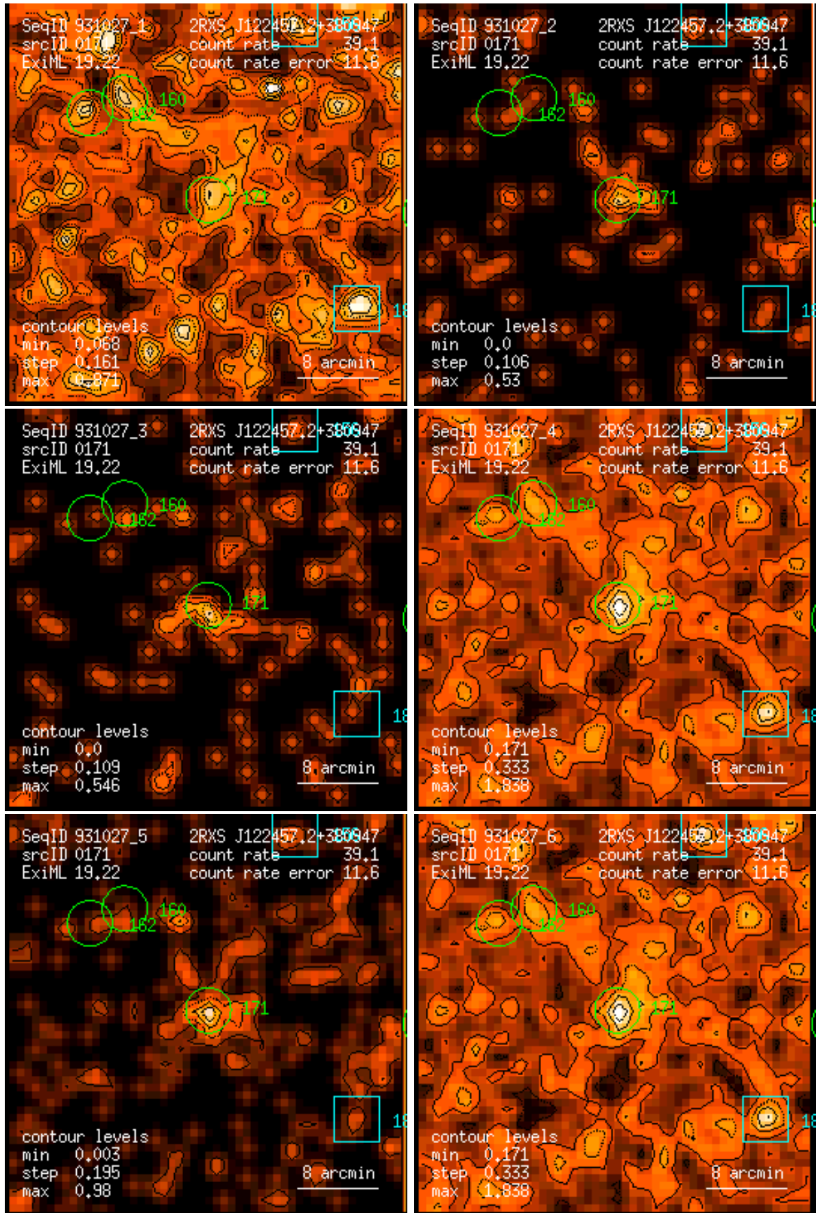
Figure 171: RASS 931027: detection 0171: band rate images, Gaussian filter: (1) PSPC channels 11 – 41, (2) 52 – 90, (3) 91 – 201, (4) 11 – 235, (5) 52 – 201, (6) 11 – 201. Broad band rates in counts/ks. Band rate contour levels in counts/ks/arcmin 2 .
